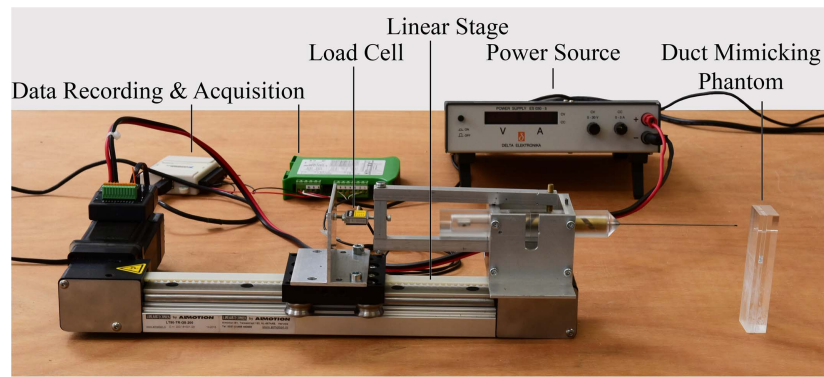
Figure 11. Measurement Facility. The measurement facility consisted of the prototype confined within an aluminum facility, the duct-mimicking phantom, a linear motion stage to actuate the cutting blades, a power source to power the motion stage, and data recording and acquisition boxes.
