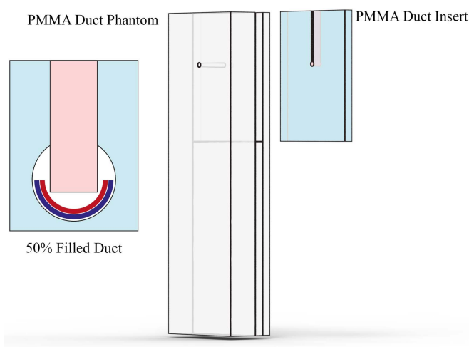
Figure 12. Milk Duct Mimicking Phantom. The breast-mimicking phantom consists of a PMMA laser-cut duct model through which a gelatin lesion phantom is inserted, which mimics a 50% filled duct. Color indications: Blue = Outer cutting blade, Light Blue = Rigid PMMA duct model insert, Light Grey = PMMA duct phantom, Pink = lesion-mimicking phantom, and Red = Inner cutting blade.
