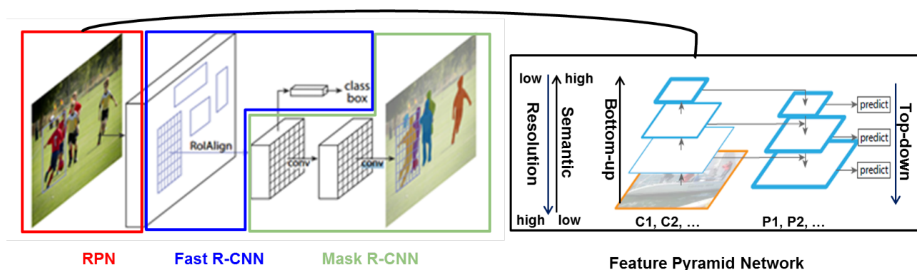
Figure 1. The framework of Mask R-CNN (He et al., 2017, Lin et al., 2017), which combines FPN, RPN and Fast R-CNN.
