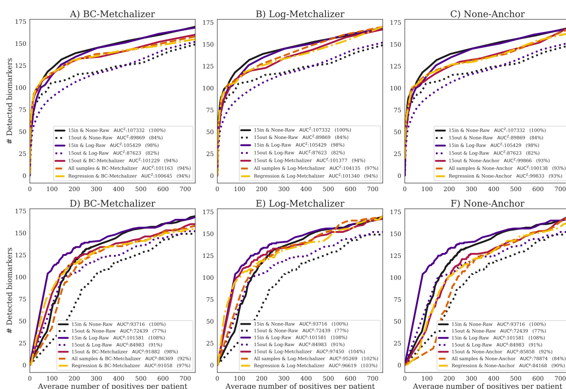
Figure 4. The number of detected expected biomarkers versus the average number of positives per patient. A curve in each (sub)figure was formed by increasing the Z-score or p -value threshold ( Z_{abnormal} , Methods). The legend indicates (per curve) the methods used to determine Z-scores and how data was normalized, the AUC and AUC expressed as percentage of the AUC_{15in\&None-Raw}^Z . Performances using (A) BC-Metchalizer and Z-scores, (B) Log-Metchalizer and Z-scores, (C) None-Anchor and Z-scores, (D) BC-Metchalizer and p -values, (E) Log-Metchalizer and p -values, and (F) None-Anchor and p -values.
