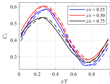
Fig. 28 Unsteady lift (solid lines) and quasi-steady lift (dashed lines) over the period at \alpha = 5^\circ for the gust with f_g = 5.7 Hz.
