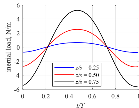
Fig. 32 Inertial loads at different spanwise locations for the gust with f_g = 3.2 Hz at \alpha = 10^\circ .
