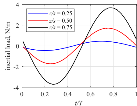
Fig. 31 Inertial loads at different spanwise locations for the gust with f_g = 5.7 Hz at \alpha = 5^\circ .
