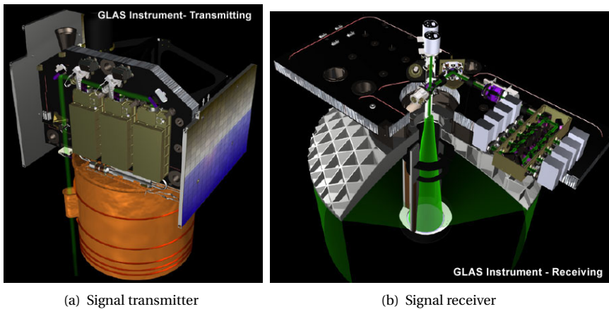
Figure 2.4: The on-board Geoscience Laser Altimeter System (GLAS) of ICESat (Credit: NASA)
