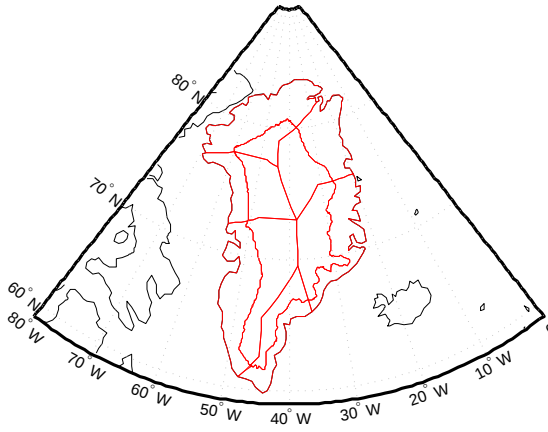
(b) 12 mascons
