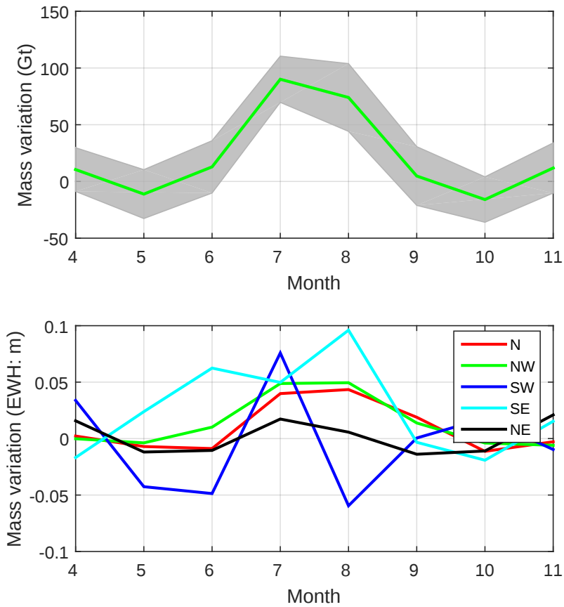
Figure 5.13: Estimates of seasonal meltwater storage, obtained as the monthly deviations from the April-May and September-November linear fit of “Total-SMB” (brown line in Fig. 5.11): for the whole GrIS (in Gt, top,) and for individual drainage systems (in meters of Equivalent Water Height, bottom). Labels along the horizontal axis represent months between April (4) and November (11). The shaded strip in the top plot shows the 2- \sigma error bar (the mean standard deviation is 23 Gt). The mean standard deviations of the estimates related to individual drainage systems are: 0.02 m (N), 0.02 m (NW), 0.06 m (SW), 0.03 m (SE), and 0.01 m (NE); they are not shown in the plot for the sake of its readability.
