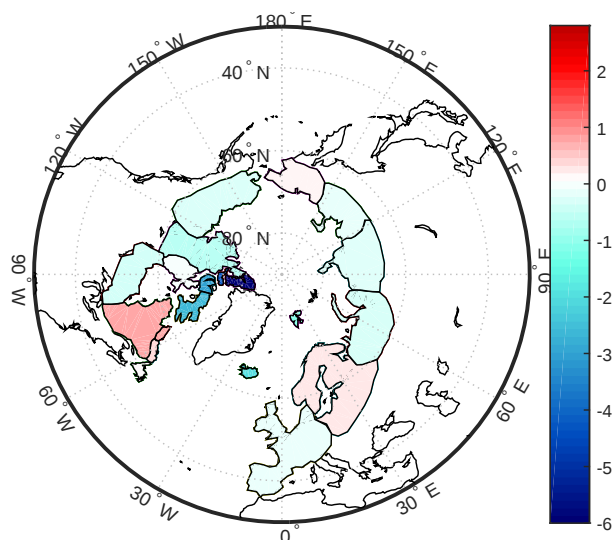
Figure 6.4: The rate of linear mass changes for mascons outside Greenland, which are introduced to simulate signal leakage (EWH: cm/yr).
