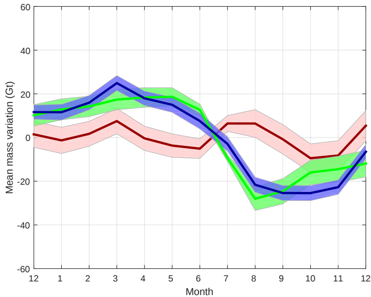
Figure 5.16: Monthly cumulative total (blue), surface (green) and residual “Total-SMB” (red) mass variations (see legend of Fig. 5.11), for drainage systems: N.
