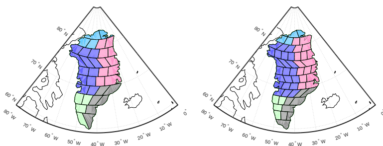
(c) 12 mascons
