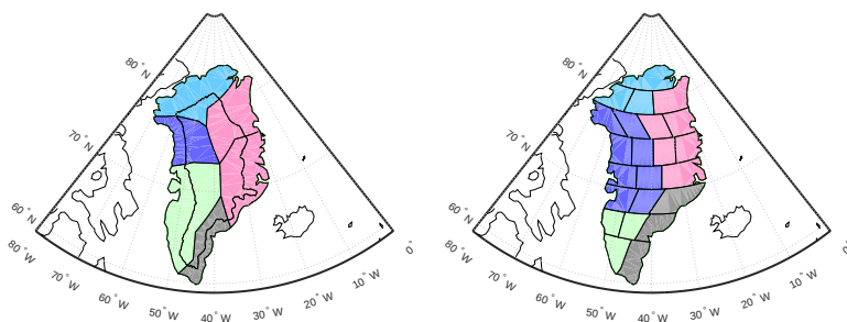
(a) 6 mascons
