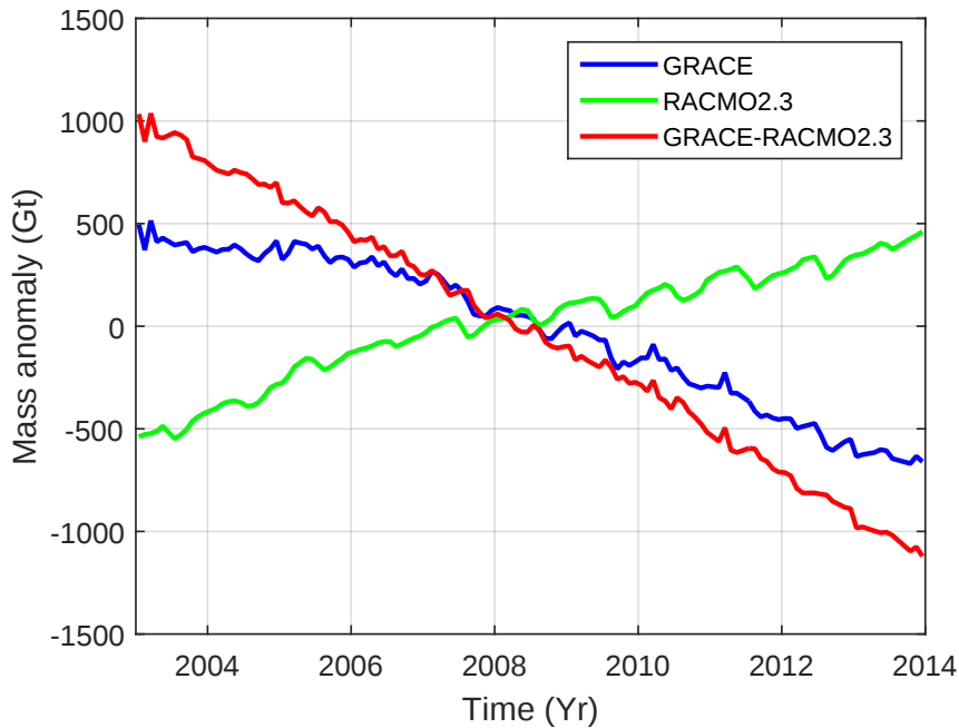
Figure 5.7: Same as Fig. 5.5, but for the NW drainage system.
