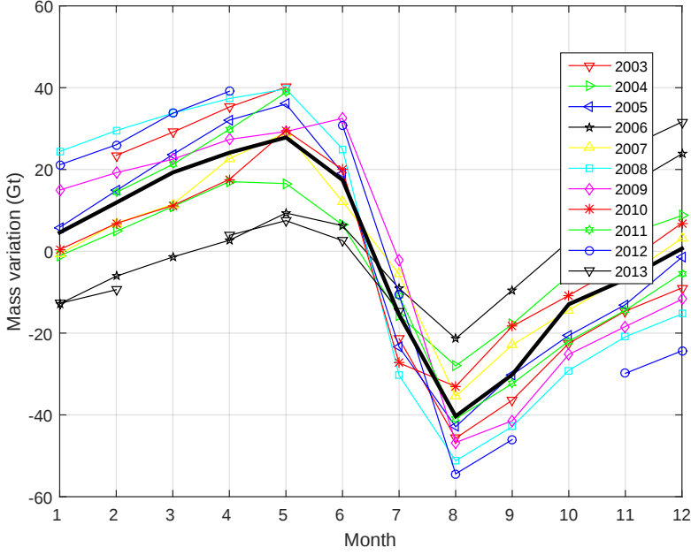
Figure 6.9: Mean SMB mass anomalies per calendar month of Greenland, \overline{m}^i (thick black curve). The thin curves represent monthly mass anomalies of different years after removing the mean yearly mass anomalies, b^j
