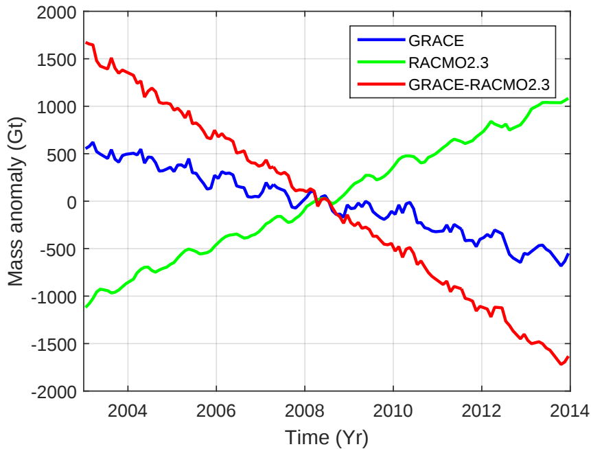
Figure 5.9: Same as Fig. 5.5, but for the SE drainage system.
