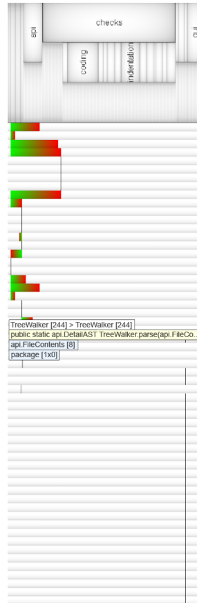
Fig. 12. Focusing on the transition between Checkstyle’s first and second phase. The tooltips provide information on the call sites.
