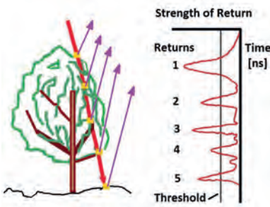
▲ Figure 2, Digitisation of multiple returns in a forest area: first, last and three returns in between (Courtesy: M. Lemmens).
