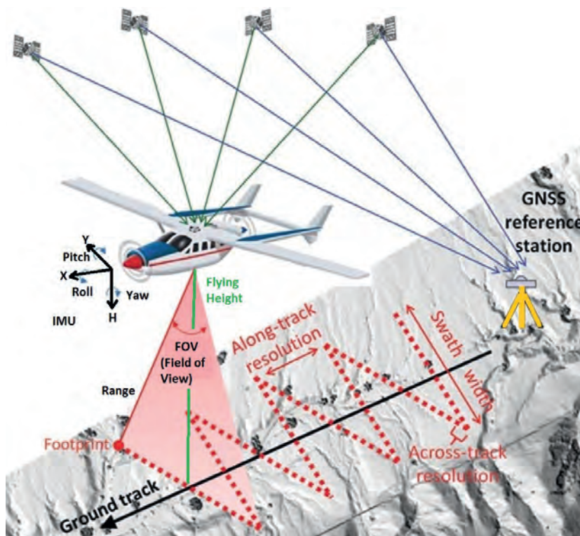
▲ Figure 1, GNSS and IMU enable automatic calculation of the X,Y,H coordinates of ground points from range and scan angle; across-track scanning is performed using a nutating mirror.
