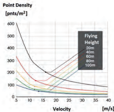
▲ Figure 4, Relationship between point density, aircraft speed and flying height of the Phoenix Alpha AL3-32 Lidar system, weighing 3.2kg.
