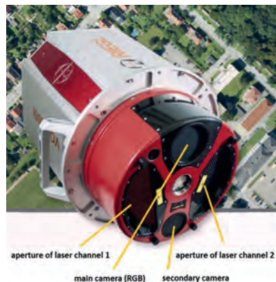
▲ Figure 5, RIEGL VQ-1560i, consisting of two laser scanners and two cameras.
