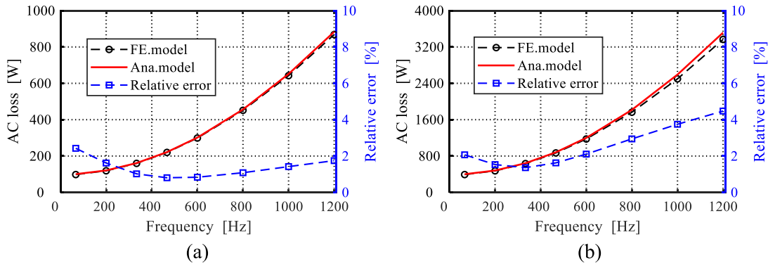
Fig. 7. Comparison of ac loss calculated by HAM and FE model of conductor arrangement a . (a) I_{\text{peak}} = 60 A. (b) I_{\text{peak}} = 120 A.
