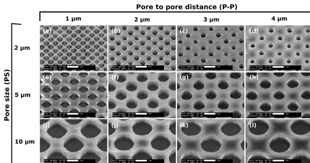
Figure 3. SEM images of the different patterned 4 \mu\text{m} -thick porous PDMS layers, with various P\text{-}P and PS , taken at a fixed magnification (8000x) and tilting angle of 26^\circ . Scale bars: 5 \mu\text{m} .
