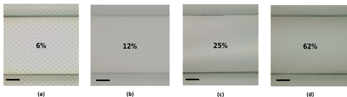
Figure 5. Optical images of 8 \mu\text{m} pore size, 4 \mu\text{m} -thick membranes of different porosities transferred to OOCs. Porosity value: (a) 6%, (b) 12%, (c) 25% and (d) 62%. Scale bars: 125 \mu\text{m} .
