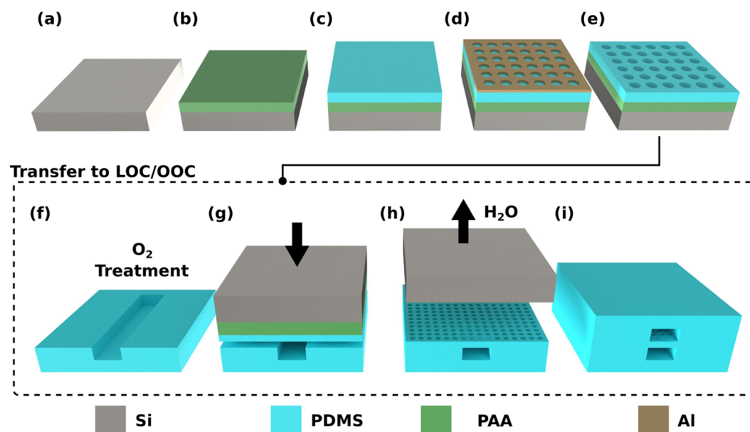
Figure 2. Schematic illustration of the microfabrication process (from (a–e)) and the transfer (from (f–i)) of the porous PDMS membranes to OOCs. (a,b) Deposition of the sacrificial and water-soluble poly (acrylic acid) (PAA) layer by spin coating. (c) Deposition of the PDMS by spin coating to define the membrane thickness. The layer is then thermally baked. (d) Deposition and patterning of the Al masking layer to define the desired pore features ( PS and P-P ). (e) Dry etching of the Al and the PDMS layers. The Al masking layer is then removed by wet etching, leaving exposed the patterned PDMS surface. (f) First step required for transferring the membrane: oxygen plasma treatment on the PDMS membrane and on the bottom surface of the PDMS-based OOCs. (g) The porous membranes, carried by the silicon substrate, are placed in contact with the activated surfaces of the OOCs and then kept under a constant pressure to promote mechanical bonding. (h) Releasing of the porous membranes by dissolving the sacrificial layer (PR or PPA) in water in an ultrasonic bath. (i) Final assembling of the OOC by attaching the top part to complete the microchannel top side.
