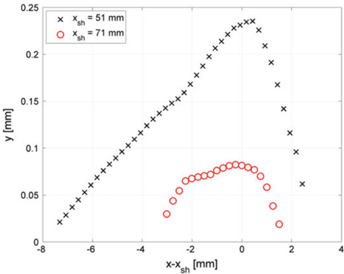
Fig. 51 Comparison between the size of the reversed flow region for an oblique shock wave reflection for a laminar and transitional incoming boundary layer
