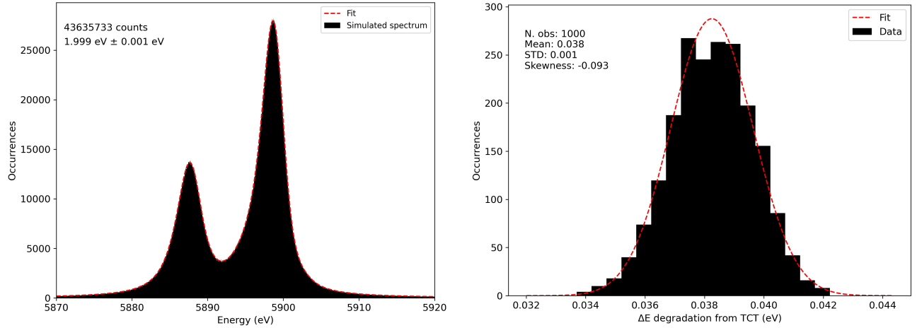
FIG. 8. Left: simulated energy spectrum for the Mn-K \alpha lines of a ^{55}\text{Fe} X-ray Perpetrator. The extreme number of simulated events is necessary to reduce the statistical error to 1 meV, since from the NEP estimation we expect the impact on resolution to be of the order of at least 10 meV. Right: histogram of the degradation in quadrature caused by random TCT in the simulated spectrum for 1000 observations.
