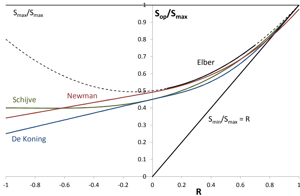
Figure 1 Illustration of various crack closure corrections proposed for the range of -1 < R < 1 [33,34,48,49,50,51,52]
