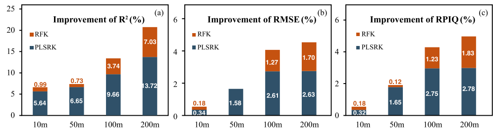
Fig. 3. Improvement for predicting SOC using PLSRK and RFK compared to PLSR and RF at four spatial resolutions.
