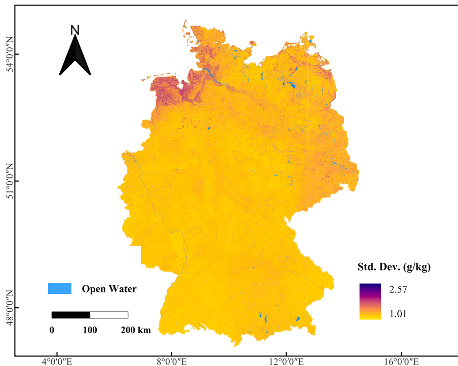
Fig. 7. The standard deviation map of SOC content in Germany by the RFK model at 100 m resolution.
