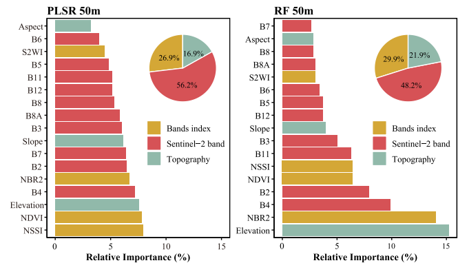
Fig. 4. Relative importance of the environmental variables used for SOC content prediction in the PLSR and RF models at 50 m spatial resolution. B2 to B12 correspond to band 2 to band 12 of Sentinel-2 data; NVDI, normalized difference vegetation index; NBR2, normalized burn ratio 2; S2WI, soil moisture index; NSSI, NPV-soil separation index.
