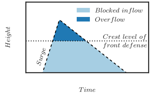
Figure 3: A front defense can block surge from flowing into a basin; however, any overflow will still enter the basin.
