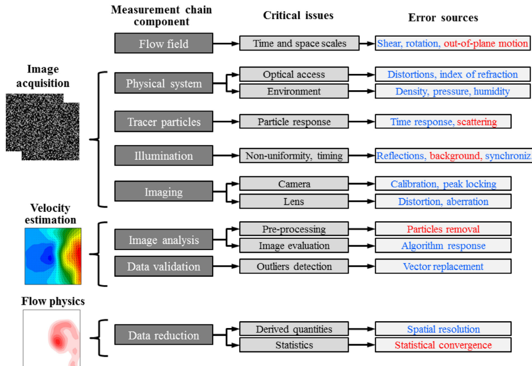
Figure 4. Schematic representations of the main components of the PIV measurement chain and the most relevant error sources. Error sources which are mainly systematic or mainly random are indicated in blue or red, respectively (it should be noted that some error sources such as peak locking are both random and systematic). Reproduced with permission from Wieneke (2017b). © 2017 B.F.A. Wieneke.
