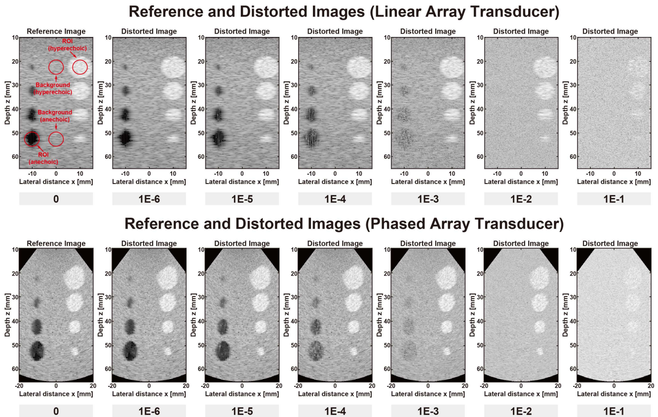
Fig. 6. Reference and distorted images for both linear array and phased array transducers at different BER levels (without error detection or correction)
