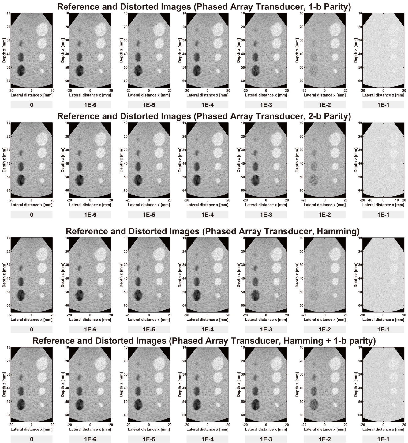
Fig. 8. Reference and distorted images for phased array transducers at different BER levels, with error detection using parity bits and error detection and correction using Hamming coding.
