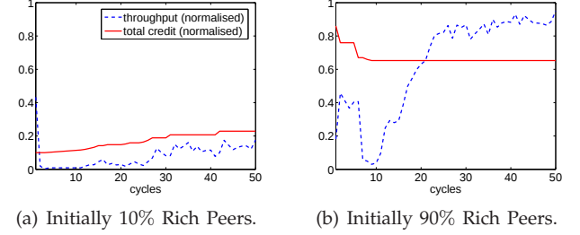
Fig. 4. The normalized throughput and credit in the system with the adaptive credit intervention mechanism.
