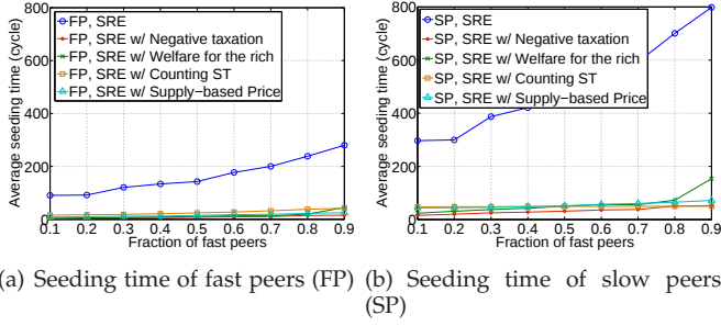
Fig. 10. Strategy performance in alleviating discrimination with 30% over-seeding peers (OSP).
