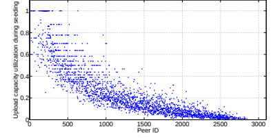
(c) Individual upload capacity utilization during seeding.
