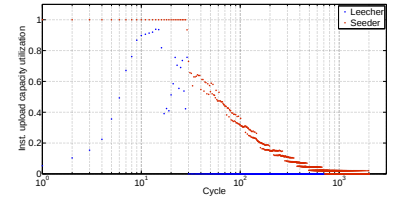
Fig. 13. The average upload capacity utilization.
