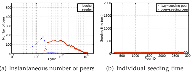
Fig. 18. SRE with counting seeding time under dynamic file popularity.
