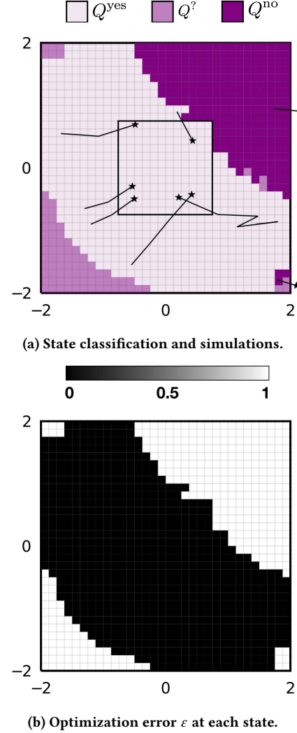
Figure 3: Synthesis results and simulations for the nonlinear system for \varphi_2 . The black square in (a) indicates the region with label Des .
