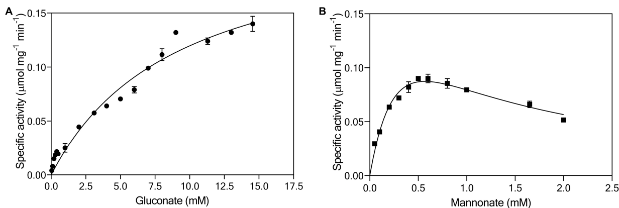
FIGURE 5 | Effect of (A) gluconate (●, mM) and (B) mannonate concentrations (■, mM) on the specific enzymatic activity ( \mu\text{mol mg}_{\text{protein}}^{-1} \text{ min}^{-1} ) of gluconate kinase and mannonate kinase, respectively, in cell extracts of L. suebicus LCV1, pre-grown on galacturonate in anaerobic chemostat cultures ( D = 0.13 \text{ h}^{-1} , 30^\circ\text{C} , pH 4). The average \pm mean deviations were derived from duplicate measurements.
