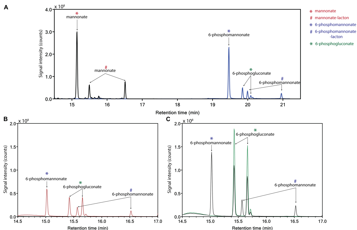
FIGURE 4 | Identification of products from the conversion of mannonate or 6-phosphogluconate, in the presence and absence of ATP, with cell extract from L. suebicus LCV1, grown on galacturonate in anaerobic chemostat cultures ( D = 0.13 \text{ h}^{-1} , 30^\circ\text{C} , pH 4). (A) 0.5 h incubation of mannonate with cell extract in the absence (black line) and presence of ATP (blue line), (B) incubation of mannonate with cell extract and ATP, start of incubation (black line), and sample taken after 3 h of incubation (red line), and (C) incubation of 6-phosphogluconate, start of incubation (green line), and sample taken after 3 h of incubation (black line). For each experiment, one of two of independent biological duplicate experiments is shown. Data for the duplicate experiments are shown in Supplementary Figure S3 . Different retention times of compounds in the panels are caused by a reduced column length for the experiments shown in C . Retention times of the standards (mannonate and 6-phosphogluconate) and the annotated GC-MS profile of mannonate are shown in Supplementary Figures S4, S5 , respectively. *sugar acid; #lacton-variant of the sugar acid.
