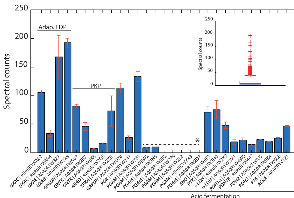
FIGURE 3 | Identified proteins from the isomerase pathway (adapt. EDP), phosphoketolase pathway (PKP) and acid fermentation plotted as normalized spectral counts in LC-MS-based proteomic analysis. The inset shows the box plot from all identified proteins within a range of 0–250 normalized counts. Only three protein hits were above this range, which are not shown. All proteins detected from the isomerase pathway, phosphoketolase pathway, and acid fermentation were above the 75th percentile of the complete proteome dataset. Bars represent the average value of two biological reactor duplicates, and error bars show the standard deviation between runs. *Paralogous genes.
