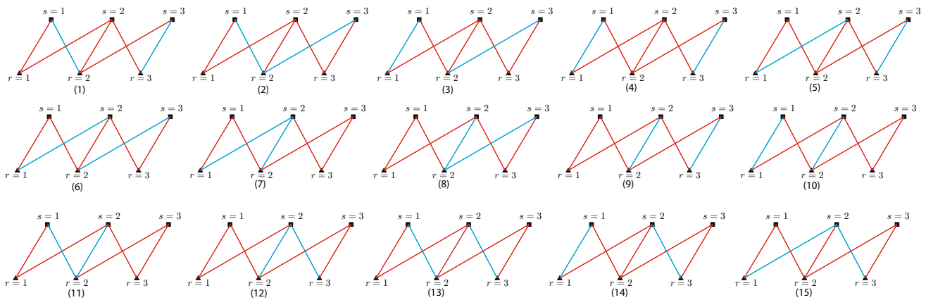
Fig. 3 All 15 spanning trees of the ambiguity graph (in red), given in Fig. 1, that represent the ‘pivot’ edges. In each case, only two ‘rover’ edges (in blue) are left
