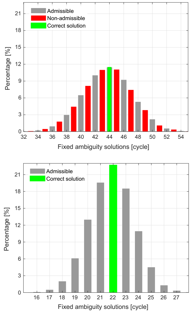
Fig. 2 Histograms of 20,000 samples of the integer-resolved ambiguity \tilde{z} = 2z_1 + 4z_2 - 6z_3 (top) compared to those of its integer-estimable version \tilde{\tilde{z}} = z_1 + 2z_2 - 3z_3 (bottom). The samples are computed using a geometry-free zero-baseline setup (Curtin CUT0-CUT2 receivers, Trimble NetR9, 4 March 2019). The DD ambiguities z_1, z_2 and z_3 correspond to the Galileo satellite pair E13–E26 on the three frequencies E1 ( z_1 ), E5a ( z_2 ) and E5b ( z_3 )
