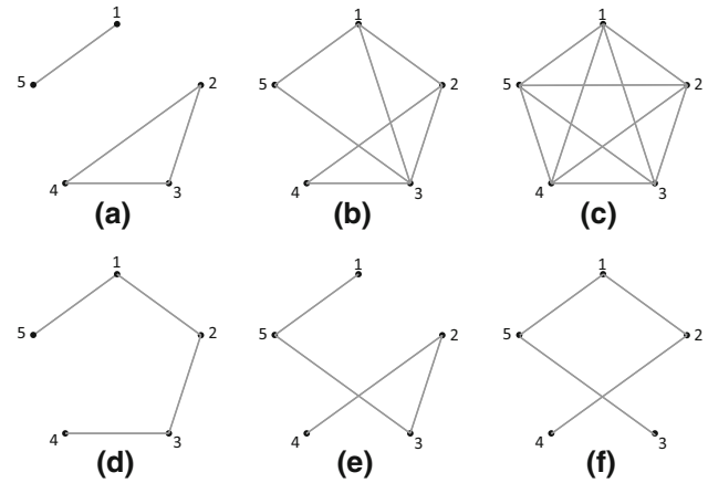
Fig. 5 Examples of connected graphs (b, c, d, e, f) compared to a graph that is not connected (a). Graph (a) is not connected because there is no path between vertices 1 and 2. Graphs (b) and (c) are connected , but not trees. They are not trees because there exist more than one path between the vertices. For instance, there exist four paths between vertices 1 and 3 in graph (b): path 1-3, path 1-2-3, path 1-5-3 and path 1-2-4-3. All the connected graphs (d), (e) and (f) are trees , since there is only one path between every two vertices
