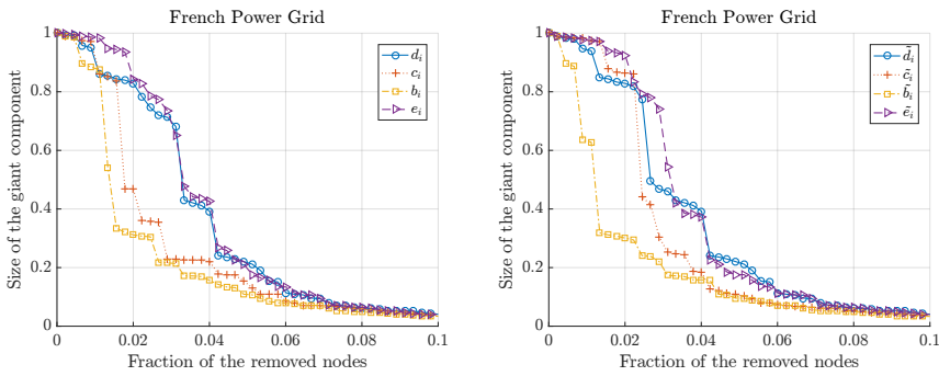
Figure 3.3: The normalized size of the giant component in the French power grid versus the removal of nodes according to the standard centrality metrics (left) and the extended centrality metrics (right). The node with optimal graph metric, computed in the resulting giant component, is removed.
