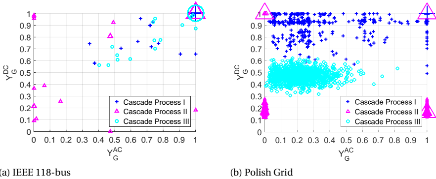
Figure 5.13: The scatter plots of the yield values under the AC vs DC cascade models for the three cascade processes initiated by single line failures. Markers are scaled according to the frequencies of corresponding data points.
