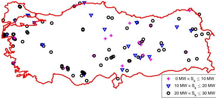
Figure 6.7: The optimal wind farm placement when f_D = 1 .
