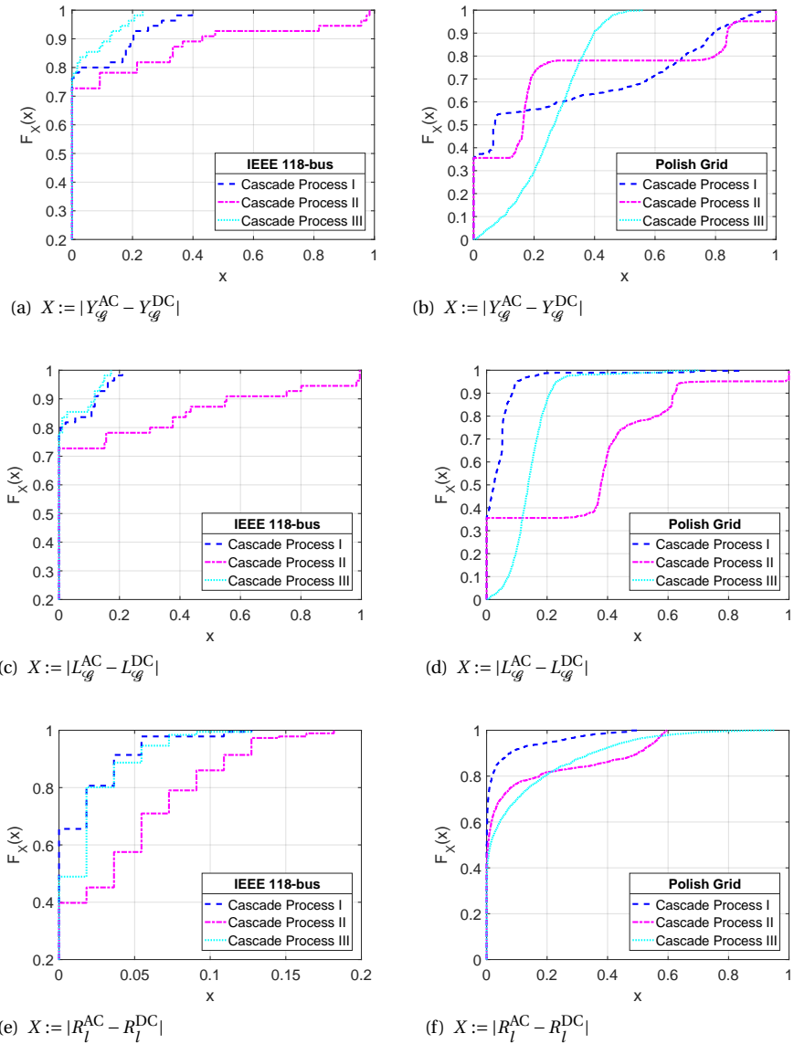
Figure 5.17: The CDFs of the differences between the metrics after cascades under the AC and DC models for the three cascade processes initiated by single line failures in IEEE 118-bus network and Polish grid.
