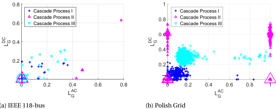
Figure 5.14: The scatter plots of the line-loss ratios under the AC vs DC cascade models for the three cascade processes initiated by single line failures. Markers are scaled according to the frequencies of corresponding data points.
