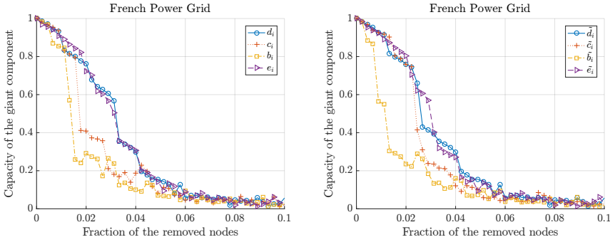
Figure 3.4: The normalized capacity of the giant components in the French power grid versus the removal of nodes according to the standard centrality metrics (left) and the extended centrality metrics (right). The node with optimal graph metric, computed in the resulting giant component, is removed.
