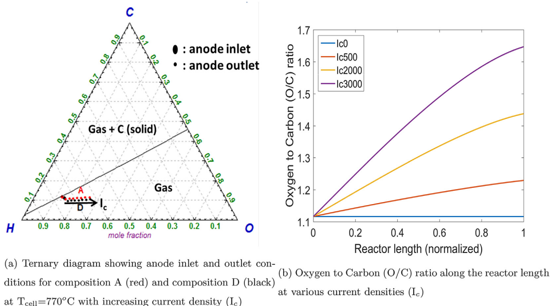
Fig. 6. Thermodynamic evaluation for carbon deposition.
