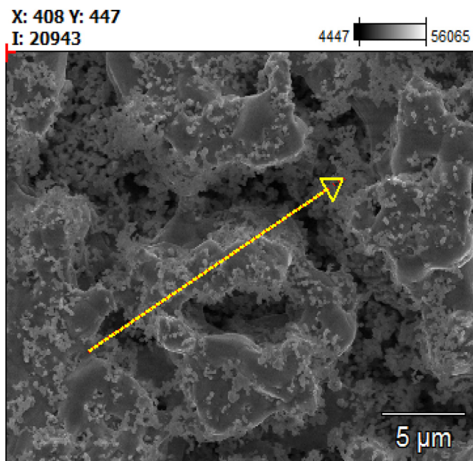
Fig. 7. SEM image of the anode cross section after experimentation.
