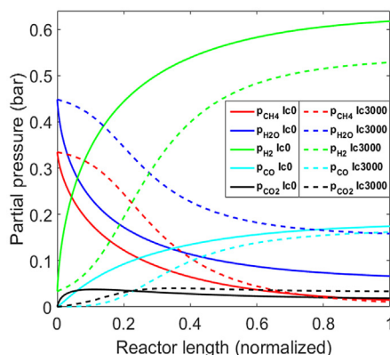
(d) Species partial pressure (bar) for open circuit ( I_{c0} ) and I_c=3000 \text{ A (m}^2\text{)}^{-1} and T_{cell}=800^{\circ}\text{C} and composition D
