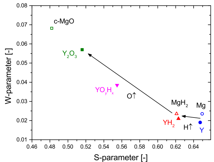
Fig. 3. S-W diagram of the S and W best-fit values for the Y, \text{YH}_{1.9+\delta} , \text{YO}_x\text{H}_y and \text{Y}_2\text{O}_3 thin films. For comparison, the S-W points for Mg and \text{MgH}_2 [19,21] thin films and c-MgO [32] are included. The arrows labeled by H↑ and O↑ indicate the trends upon increased hydrogen and oxygen insertion, respectively.
