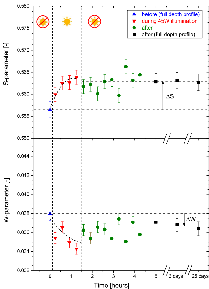
Fig. 7. (Color online only). Time dependence of the S and W parameter monitored at a fixed positron implantation energy of 6 keV during (red) and after (green) heating to T \sim 96^\circ\text{C} by 45 W illumination with a QTH lamp inside the sample chamber for a photochromic \text{YO}_x\text{H}_y film on \text{f-SiO}_2 . The blue and black data points correspond to VEPFIT fitting results obtained from full PAS depth profiles acquired before and several days after the in-situ illumination. The dashed curves serve as a guide-to-the-eye. (For interpretation of the references to color in this figure legend, the reader is referred to the web version of this article.)
