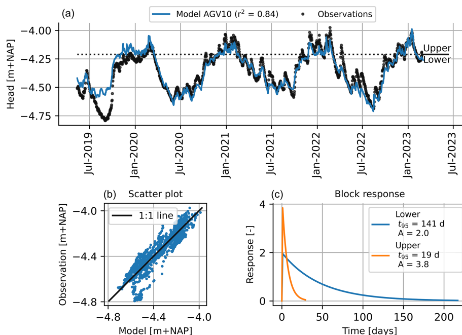
Figure 6. Illustration of the simulated head levels with the time series model in comparison with the observations for dike AGV10. Panel (a) shows the observations and model series where also the upper and lower regime are indicated with the black dotted line, and panel (b) shows the scatterplot of observed and simulated heads. Panel (c) shows the impulse response functions of the upper and lower regimes, including the parameters of the peak of the block response ( A ) and the response time ( t_{95} ) in the legend.
