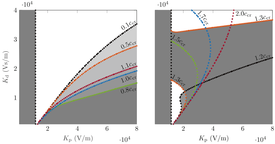
Fig. 3 Stability vs control gains for different vehicle velocities, namely v = 0.1\text{--}1.1c_{cr} (left panel) and v = 1.2\text{--}2c_{cr} (right panel); grey indicates instability. Note that for v = 1.5\text{--}2c_{cr} , the instability region is outside the closed ovals and does not have a grey background to avoid cluttering the figure
