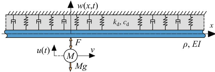
Fig. 1 System schematics: an infinite Euler–Bernoulli beam continuously supported by a viscoelastic foundation subject to a moving mass. The vehicle–structure interaction is governed by the nonlinear electro-magnetic suspension
