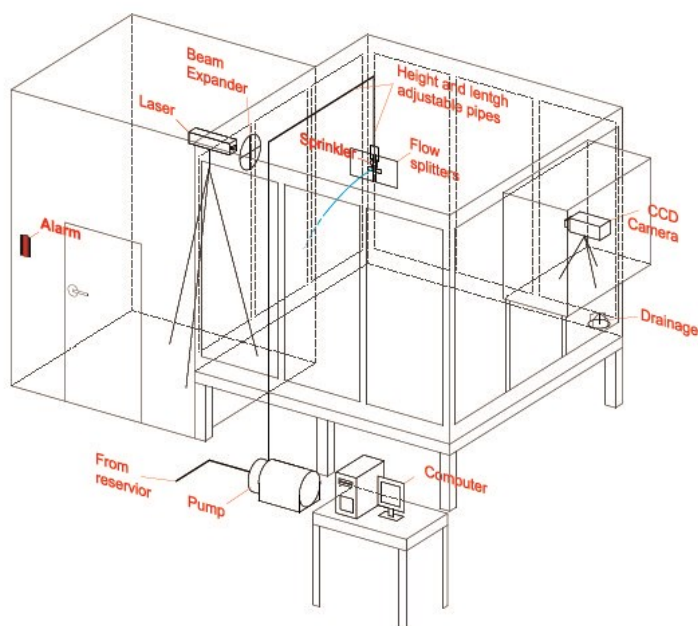
Figure 3-3 Experimental rig
