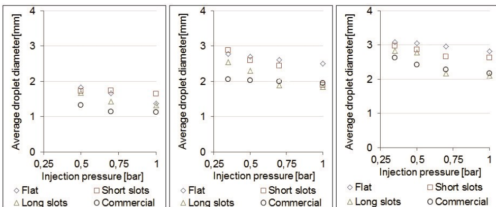
Figure 3-11 Average drop diameter for the fast response sprinkler with massive frame arms. Left: Measurements for the sprinkler head with orifice diameter d_0 = 3 mm. Middle: Measurements for the sprinkler head with orifice diameter d_0 = 4 mm. Right: Measurements for the sprinkler head with orifice diameter d_0 = 6 mm
