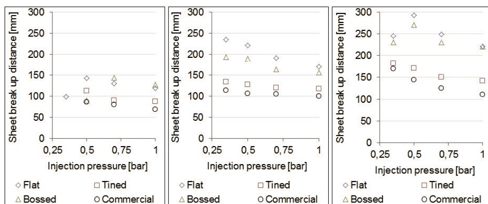
Figure 3-7 Breakup distance of the liquid sheets for the fast response sprinkler with thin frame arms. Left: Measurements for the sprinkler head with orifice diameter d_0 = 3 mm. Middle: Measurements for the sprinkler head with orifice diameter d_0 = 4 mm. Right: Measurements for the sprinkler head with orifice diameter d_0 = 6 mm
