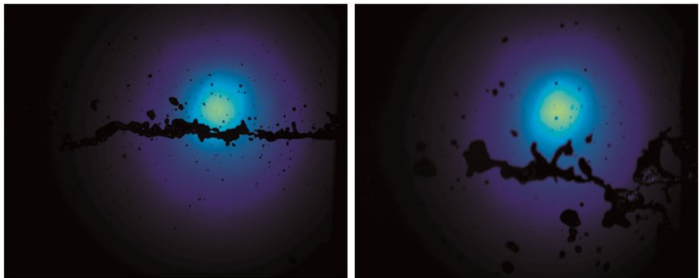
Figure 3-14 Sheet leaving the flat deflector of the sprinkler with massive frame arms. Orifice diameter d_o=6 and injection pressure of 0.5 bar. Left: Sheet formed between frame arms. Right: sheet formed behind the frame arms (after striking the frame arm).
