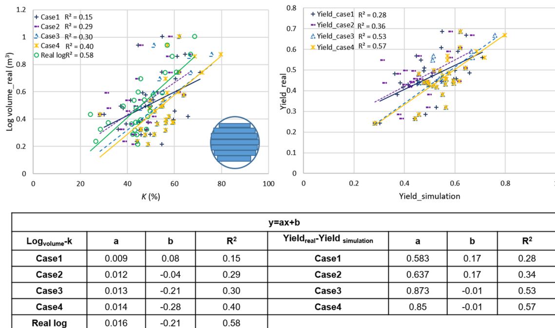
Fig. 6 Relation between actual and virtual log volumes and yield ( k ). Constants (a, b) of the linear correlations and the resulting R^2 values are shown in the table below each figure
