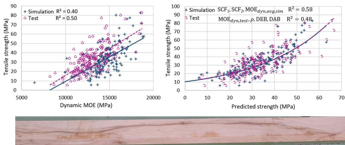
Fig. 8 Comparison of the tested and simulated parameters to the measured tensile strength and an example of beech board with extreme fiber deviation. (Left: simulated vs. actual dynamic MoE, right: predicted vs. actual tensile strength of the boards)
