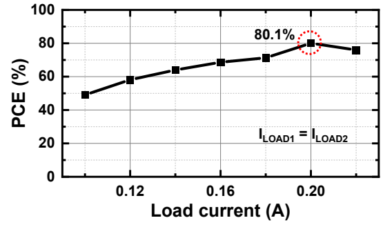
Fig. 9. Post-layout simulated PCE of the proposed dual-output rectifier.
