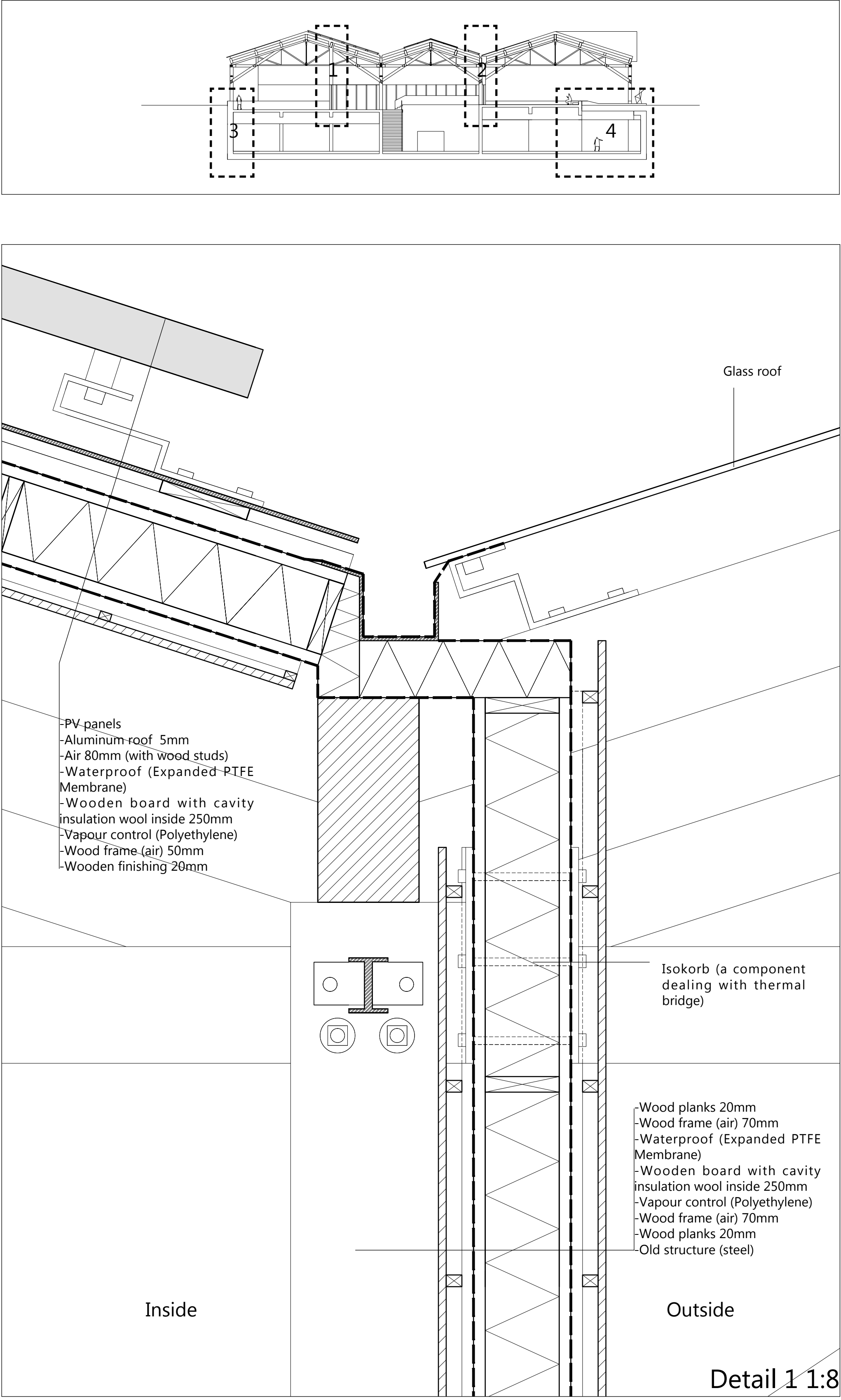
Detail 1 1:8
