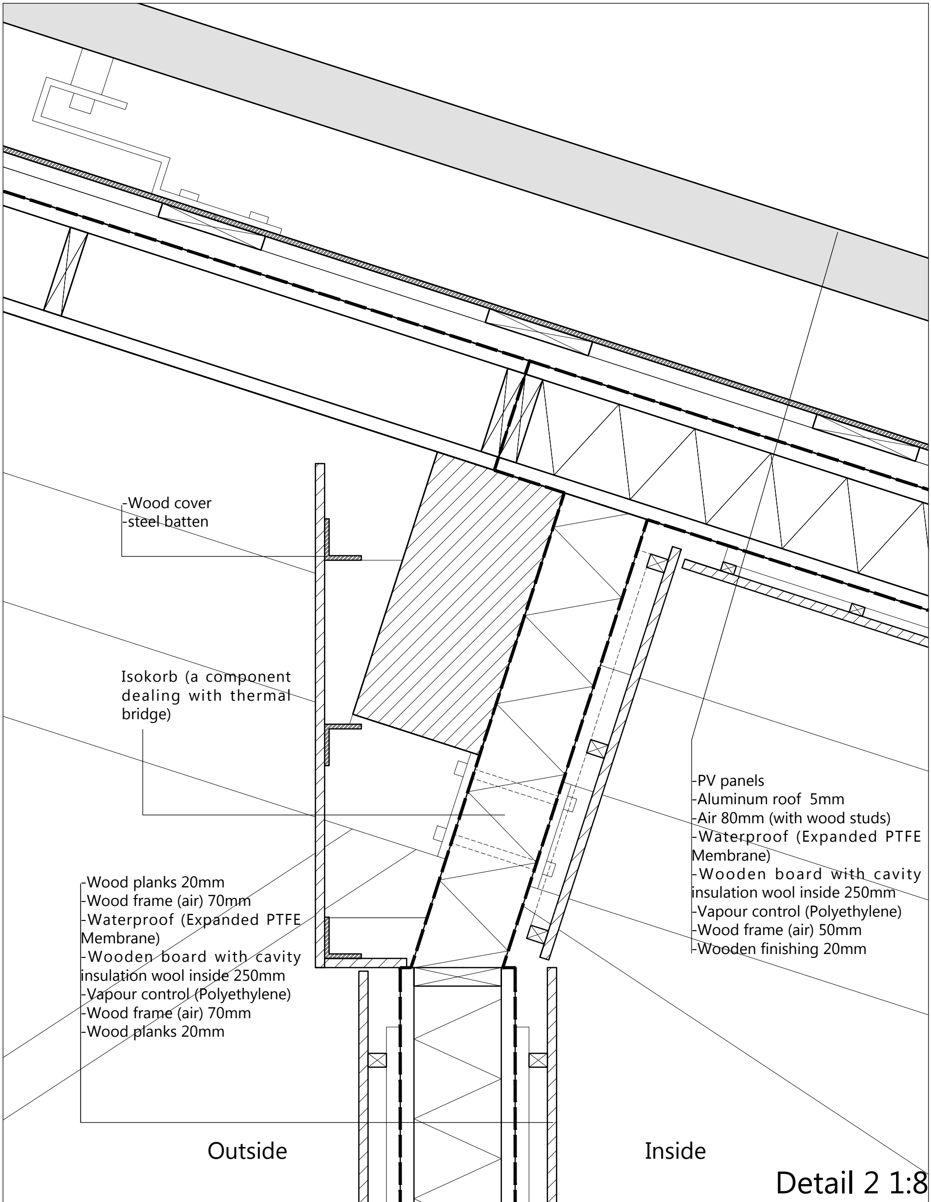
Detail 2 1:8
