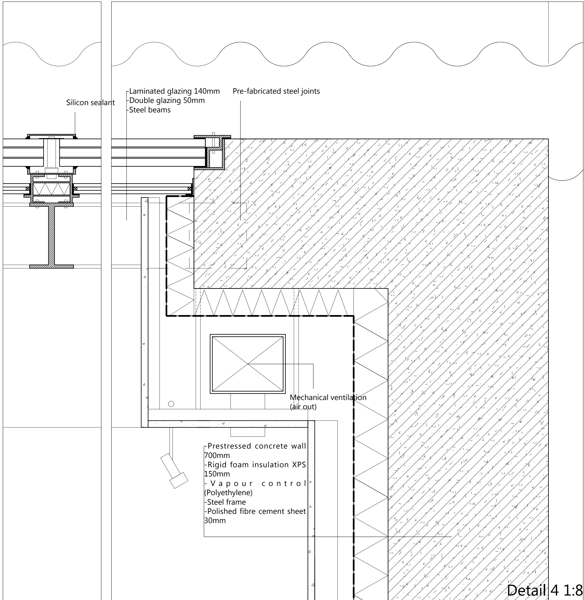
Detail 4 1:8
