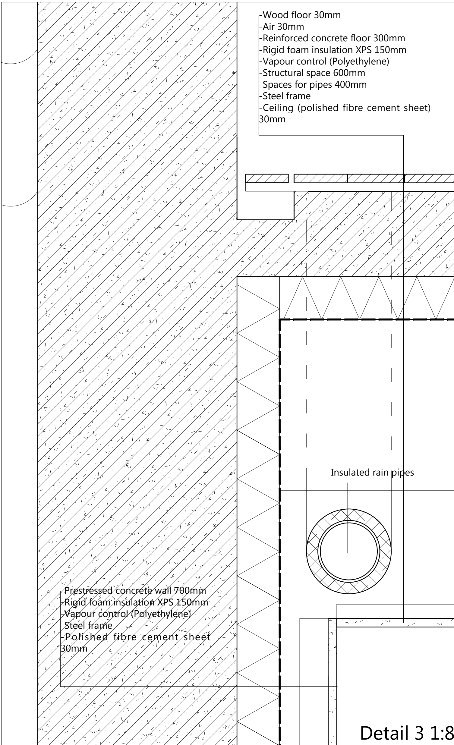
Detail 3 1:8
