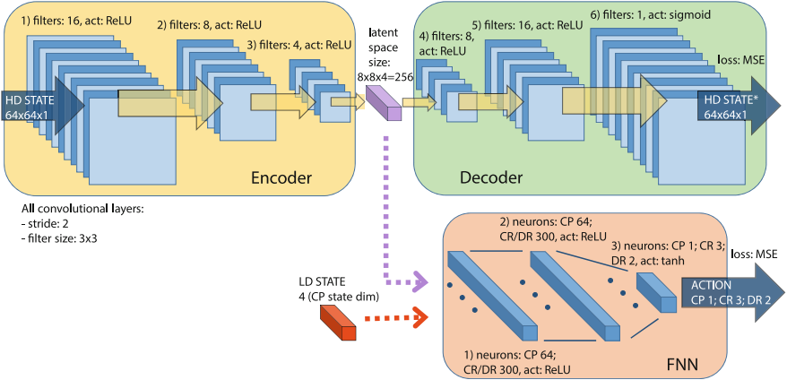
Fig. 1. D-COACH neural networks architecture. Variations between environments are specified with the acronyms CP (Cart-Pole), CR (Car Racing) and DR (Duckie Racing). HD STATE: high-dimensional state space. LD STATE: low-dimensional state space.
