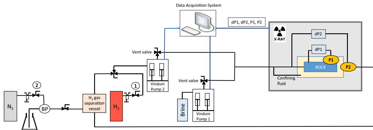
Figure 2. Schematic of experimental apparatus.
