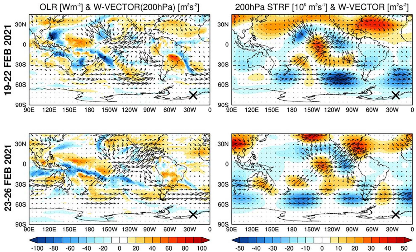
Figure 3. (a) Outgoing longwave radiation (shading; \text{W m}^{-2} ) and 200 hPa W vectors (arrows; \text{m}^2 \text{s}^{-2} ) averaged over 19–22 February 2021. (b) is as (a) but with the shading giving the 200 hPa stream function anomalies ( 10^6 \text{ m}^2 \text{s}^{-1} ) with respect to the 1979–2020 ERA-5 climatology. (c) and (d) are as (a) and (b) but with the fields averaged over 23–26 February 2021. The cross in all panels indicates the approximate location of the Brunt Ice Shelf (BIS).
