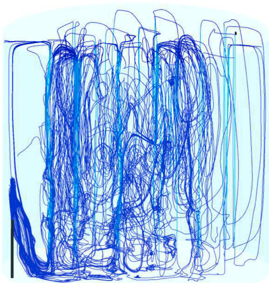
Fig. 7. Schematic streamlines (starting from the sludge feed location) in the whole digester filled with different sludge sources, (A) the locally treated sewage sludge; and (B) referred manure slurry [18,19].
