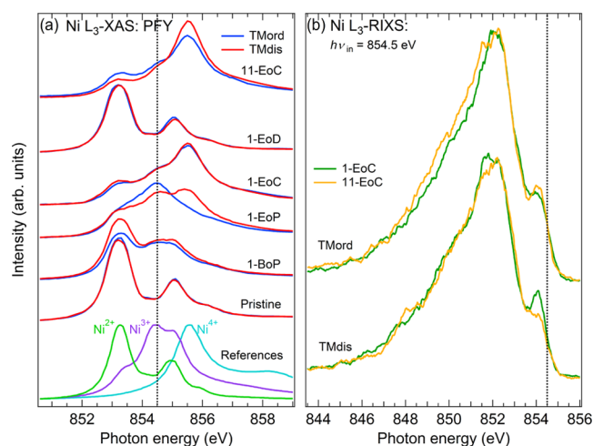
Figure 5. (a) Ni L 3 -edge XAS in PFY signal of cycled LNMO electrodes harvested from half-cells at different SOC. Reference spectra as reported by Qiao et al. 49 (b) Ni L 3 -edge RIXS at an incident photon energy of 854.5 eV of the 1st and 11th cycle delithiated SOC.
