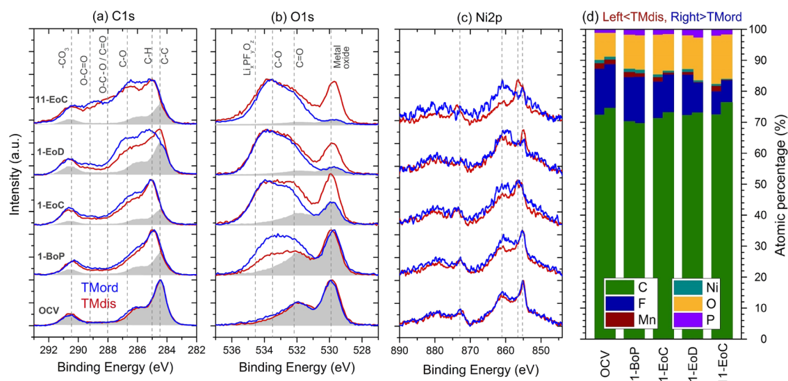
Figure 4. XPS results of cycled LNMO electrodes (at 55 °C) harvested from half-cells at different SOC levels (as shown in Figure 3). Normalized spectra for C 1s, O 1s, and Ni 2p are shown in (a–c), respectively. Spectrum of OCV sample (disordered) is shown in gray to enable an easier comparison (its intensity is normalized with the parts of the spectrum where bulk components are present). Relative atomic percentages of the analyzed elements are given in (d). In this figure, the left part of the bars corresponds to atomic percentages of disordered samples, while the right part is for ordered samples. “OCV” samples are obtained by electrodes harvested from half-cells after 10 h waiting time at 55 °C, but without applying any current.
