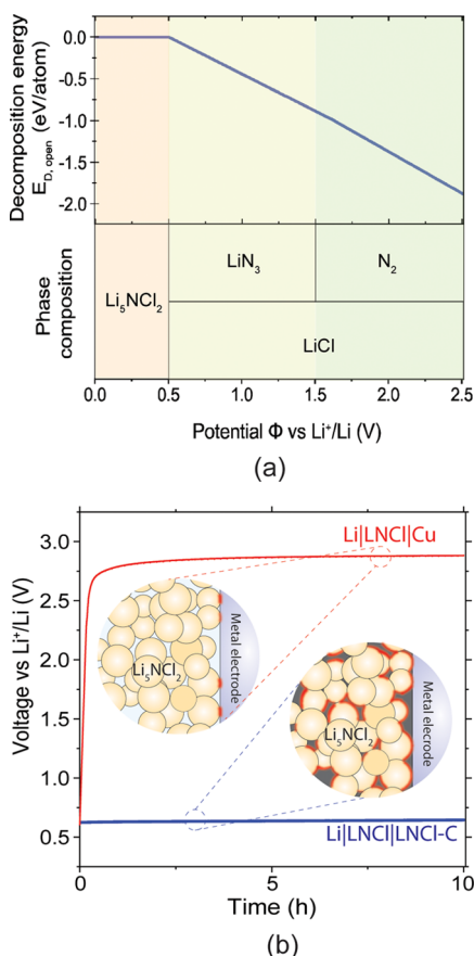
Figure 4. (a) Phase equilibria of the \text{Li}_x\text{NCl}_2 ( \{x \in \text{R}|x \geq 0\} ) phase space at different potentials \phi versus \text{Li}^+/\text{Li} . Additionally, this figure shows the decomposition energy E_{\text{D,open}} as defined by Zhu, He, and Mo 52 of LNCl at different \phi . (b) Galvanostatic oxidation of a composite LNCl-C cathode and of LNCl in contact with an ion-blocking Cu disk. The two schematics represent the cathode compositions. In the case of LNCl-C composite cathodes, the contact area with the electronic network is much larger, as sketched by the red highlighting. The constant current for both curves in (b) was 0.5 \mu\text{A} ( 0.64 \mu\text{A cm}^{-2} ).
