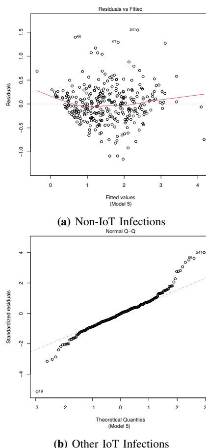
Figure 8: Residuals Plot and QQ-plot for model 5 reported in Table 2.
