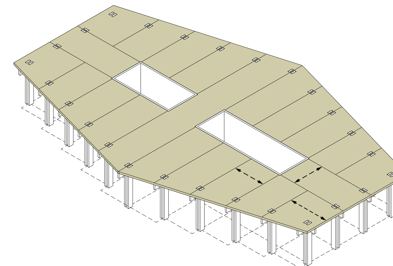
CLT floor
