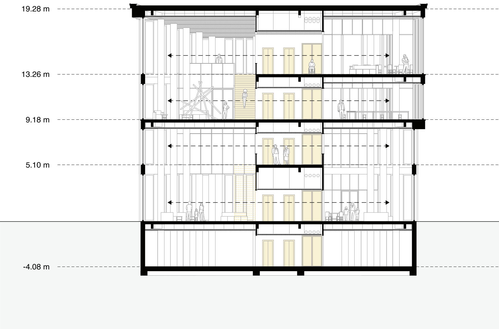
North - south section
