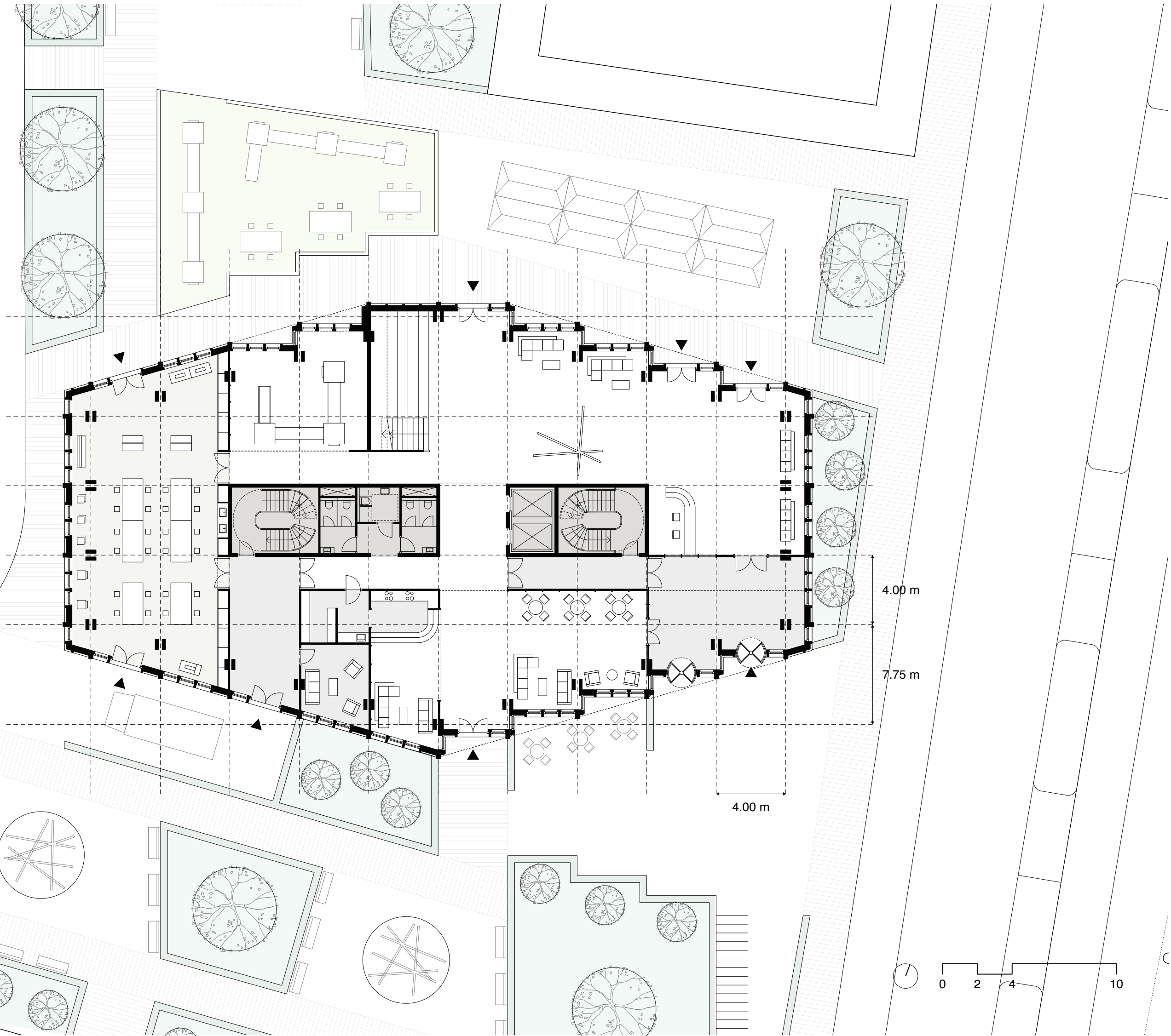
Functional organisation
