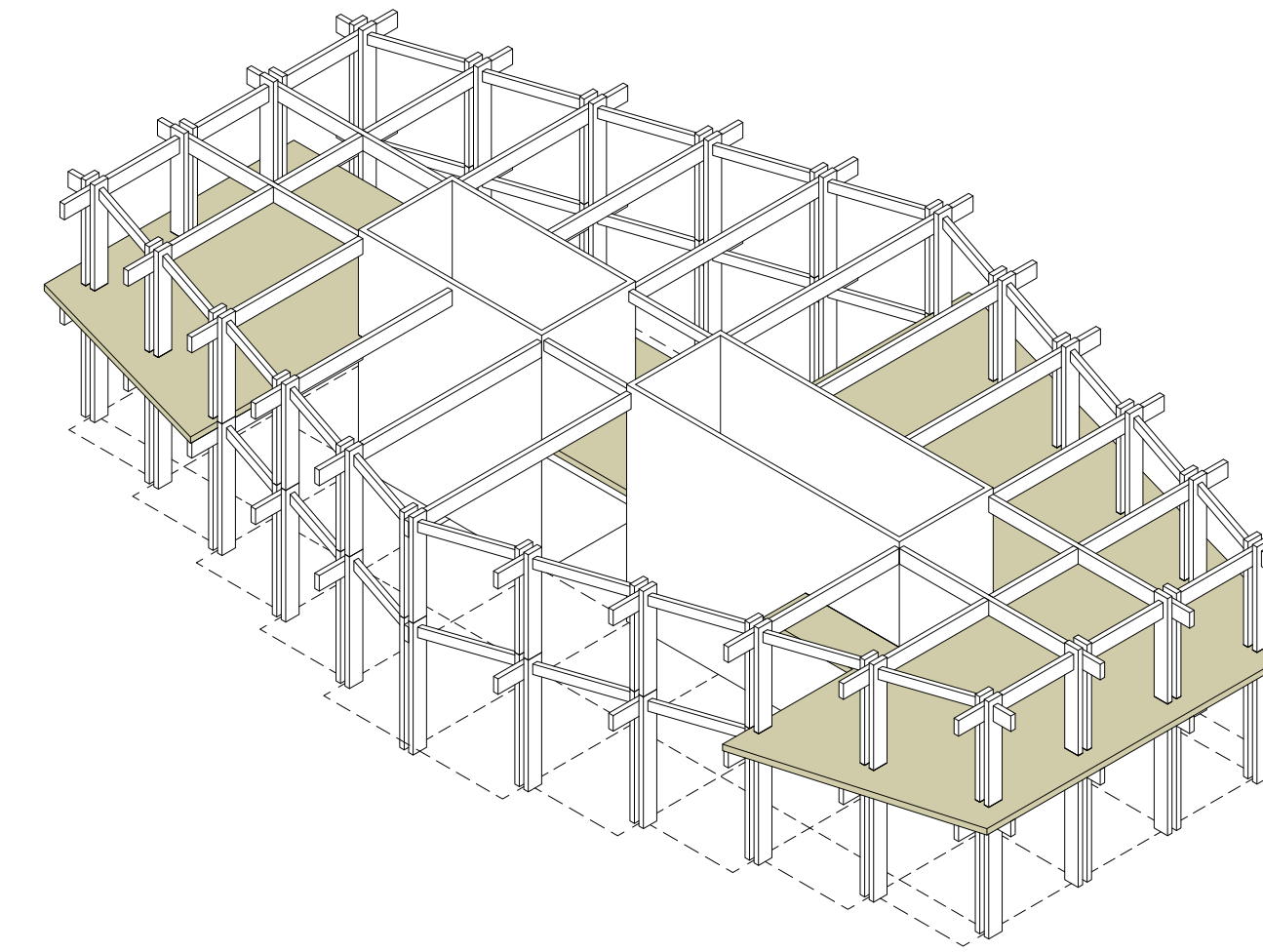
Cut voids
