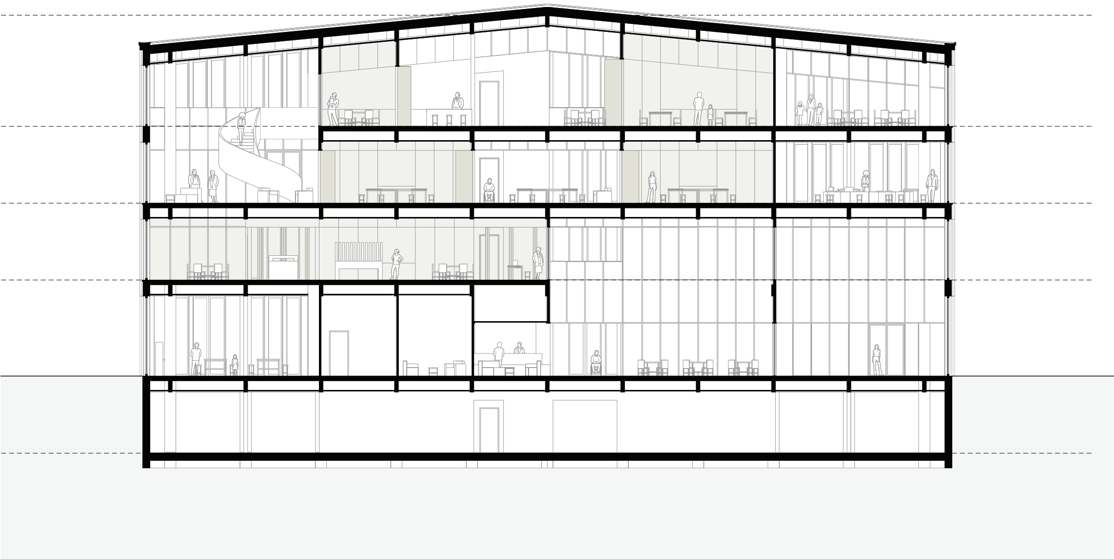
West - east section
