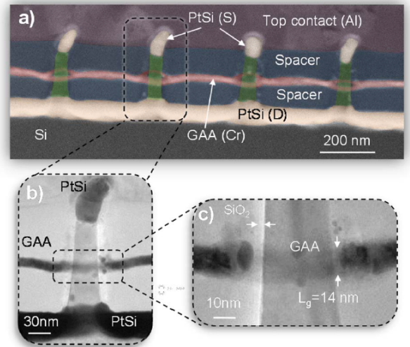
Fig. 8: VNWET device from [31]: (a) STEM image in cross section of the vertical transistor implemented in nanowire arrays, (b) single VNWET showing its (c) gate formation
