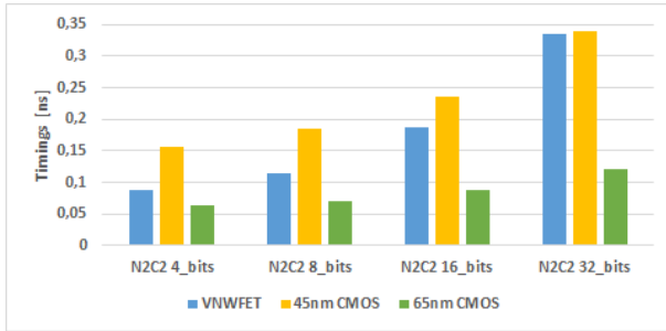
Fig. 10: VNWFET timing results vs 45/65 nm CMOS libraries
