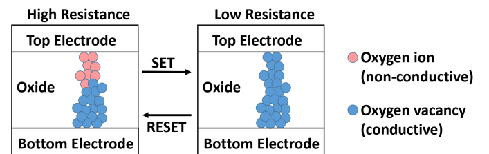
Fig. 12: RRAM technology.
