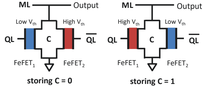
Fig. 3: Circuit of the FeFET-based Ternary Content Addressable Memory (TCAM) cell implementation. A complementary write scheme stores logic 0 and 1 in a cell.
