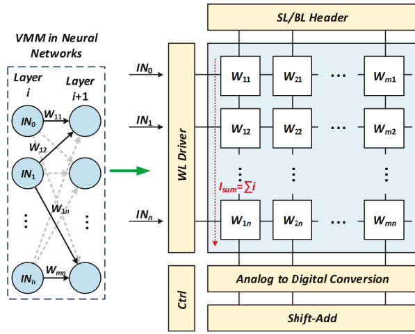
Fig. 1: Computation-In-Memory architecture [7].
