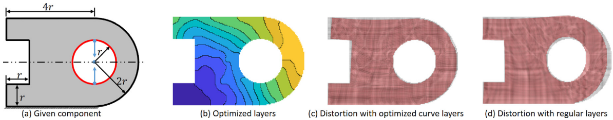
Fig. 12. The fabrication sequence of a 2D bracket (a) is optimized to minimize the average displacement of nodes on the inner circle (red). The fabrication starts from the bottom-left corner. The objective is reduced to 0.768 (c) from 10.814 (d). (For interpretation of the references to colour in this figure legend, the reader is referred to the web version of this article.)
