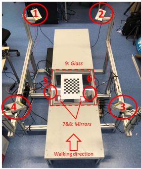
FIGURE 1. The TU Delft 4D foot Scanner with six Microsoft Azure Kinect DK cameras to capture the 4D foot shape.
