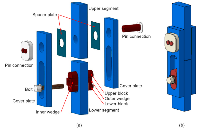
Fig. 8. CAD graphs of the C1 Wedge Connection: left in an explosive view, and right in an assembly view.
