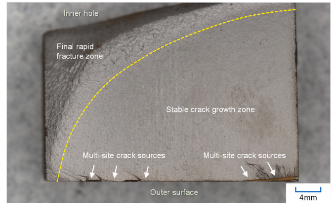
(b) OBL07: 40–350 kN, 12 Hz, 491,824 cycles
