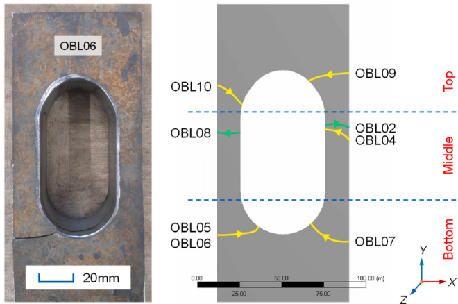
Fig. 11. Crack growth path summary of holed thick plates without surface polishing.
