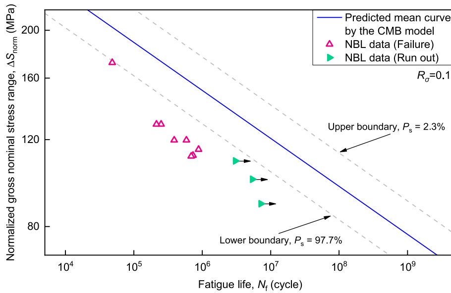
(a) CMB model-based
