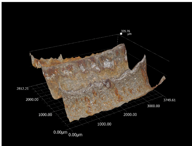
Fig. 14. Micro notch observation on the exterior surface (OBL07).
