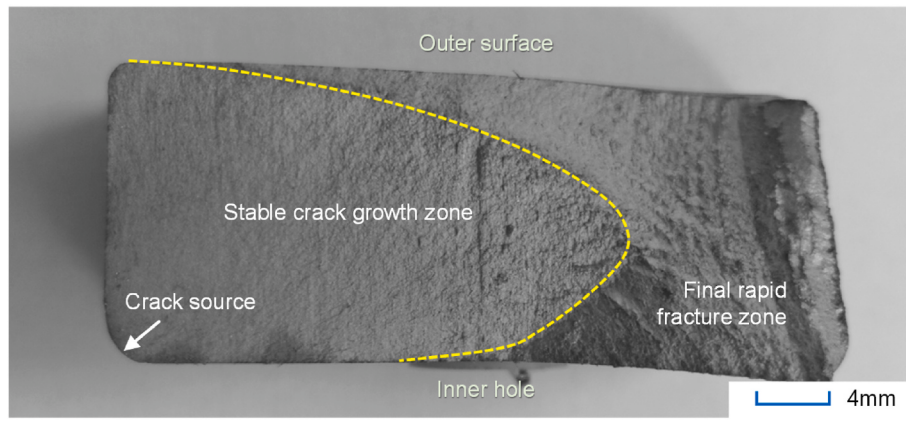
(a) NBL03: 45–450 kN, 5 Hz, 213,987 cycles
