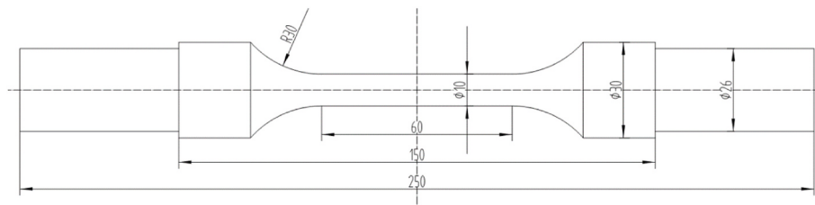
Fig. 5. Geometry and dimensions of the uniaxial tension specimen (mm).
