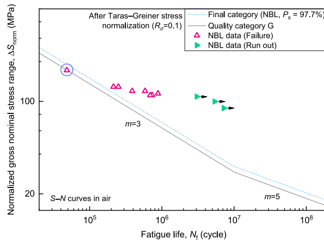
(c) DNV-RP-C203 [57]
