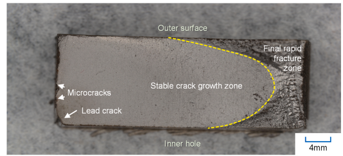
(a) OBL08: 30–310 kN, 12 Hz, 615,604 cycles
