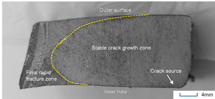
(b) NBL06: 40–400 kN, 5 Hz, 833,595 cycles
