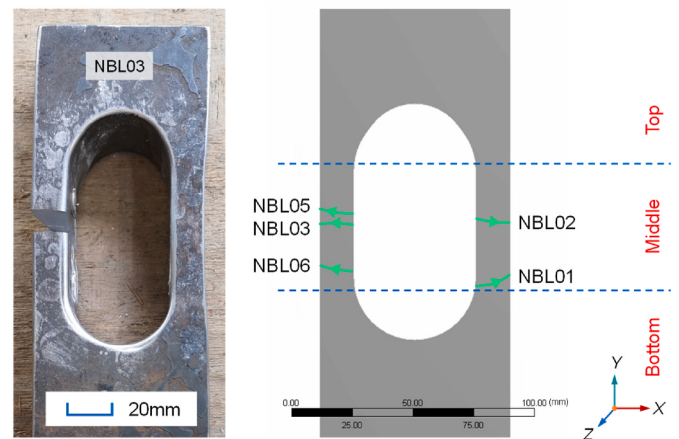
Fig. 19. Crack growth path summary of fractured holed thick plates after surface polishing.
