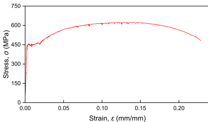
Fig. 6. Monotonic stress-strain curve.
