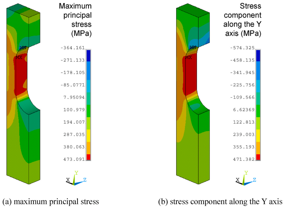
Fig. 27. Stress distributions at the load peak substep (140 MPa gross nominal stress).
