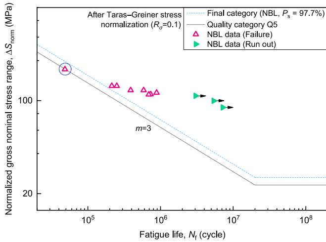
(b) BS7910-2019 [56]
