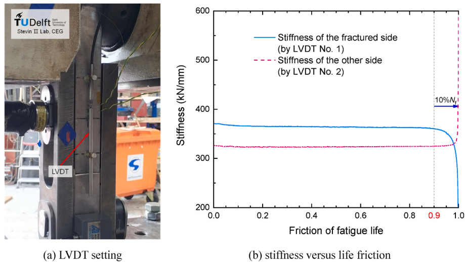
Fig. 28. Stiffness plot during the test (NBL02).
