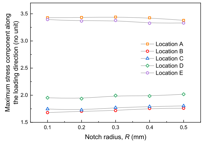
Fig. 16. Maximum notch stress in different locations and sizes.
