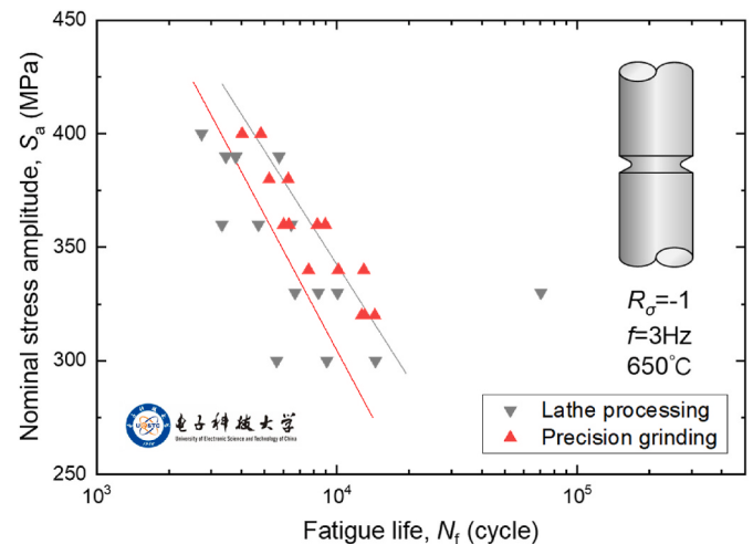
Fig. 21. Fatigue performances of GH4169 V-notched specimens processed by different techniques.
