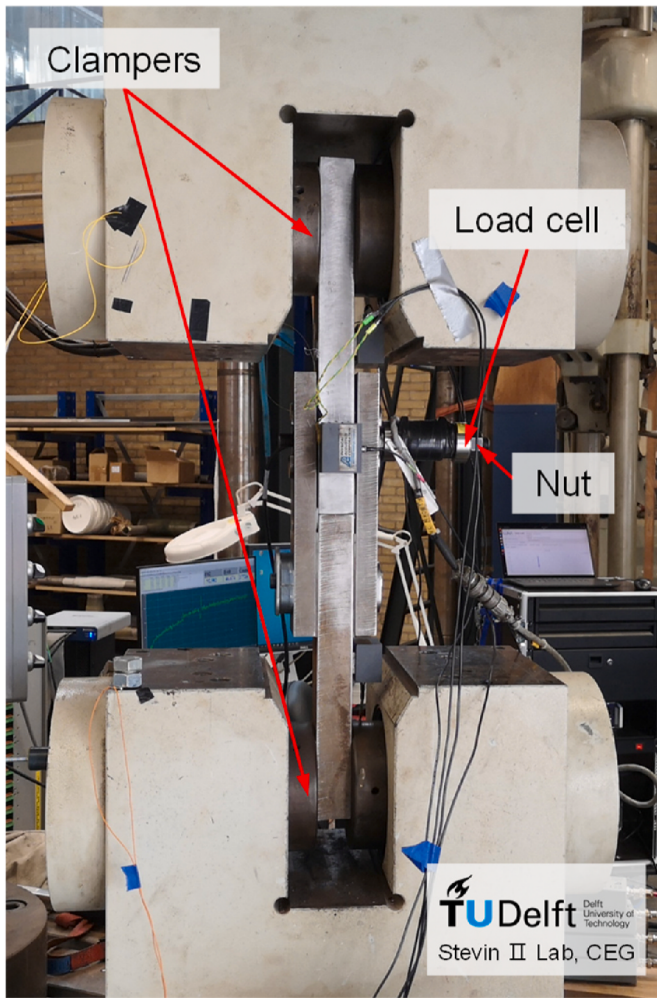
Fig. 9. Experimental setting.
