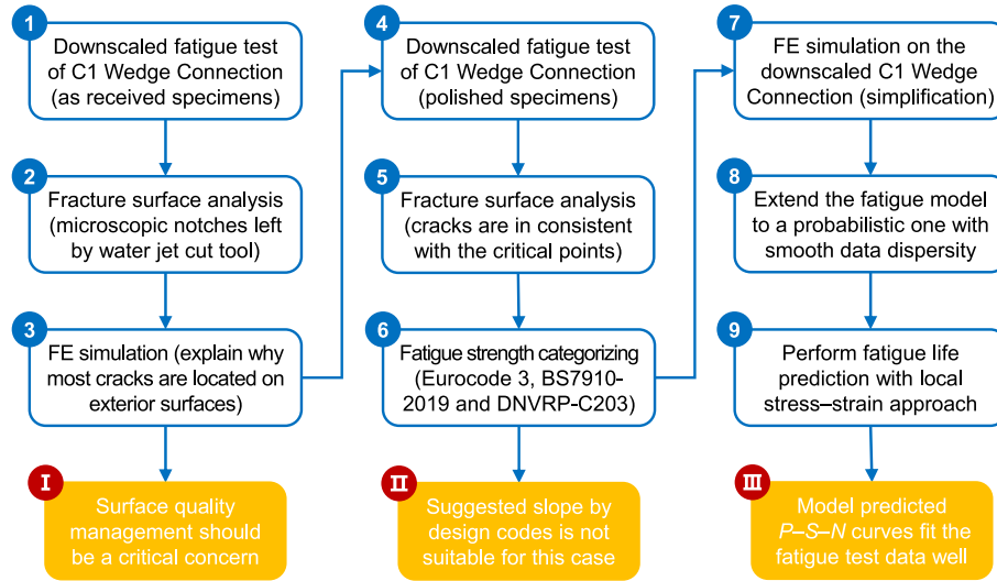
Fig. 4. The flowchart of this work.
