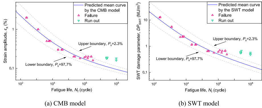
Fig. 25. Probabilistic fatigue modelling (material tests).
