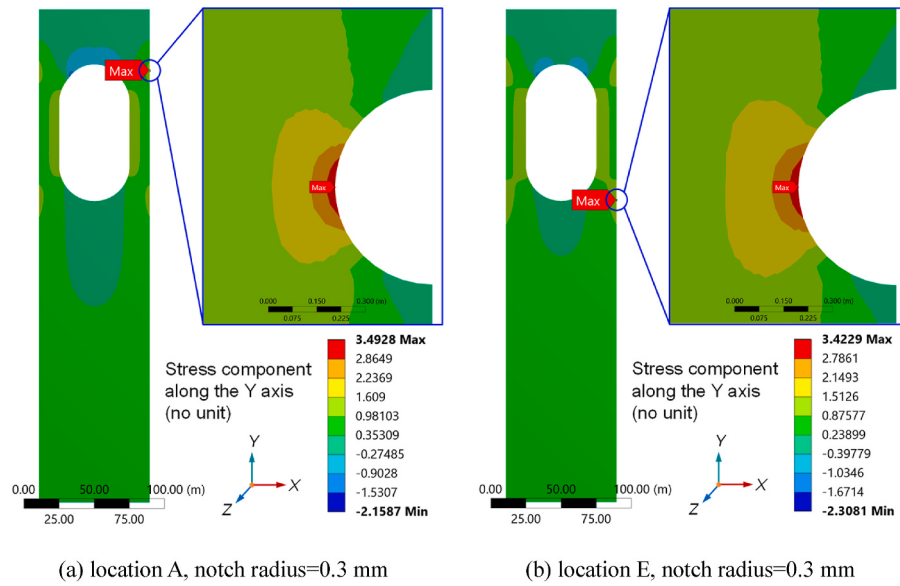
Fig. 17. Distributions of the maximum stress component along the load direction.
