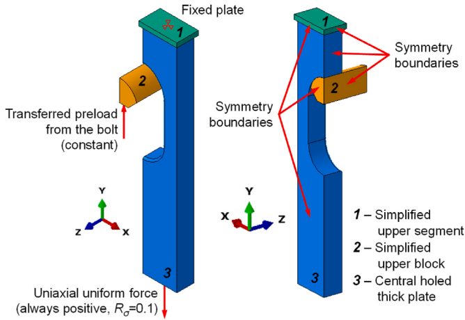
Fig. 26. Boundary and load conditions in FE simulation.
