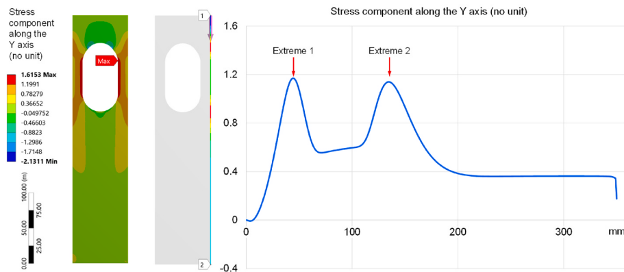
Fig. 18. Stress distribution along the path (from point 1 to 2) without any micro notch.
