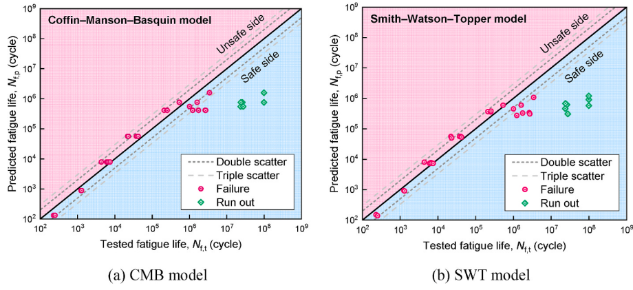
Fig. 24. Predicted versus tested fatigue lives.
