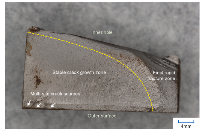
(c) OBL09: 34–314 kN, 12 Hz, 733,307 cycles
