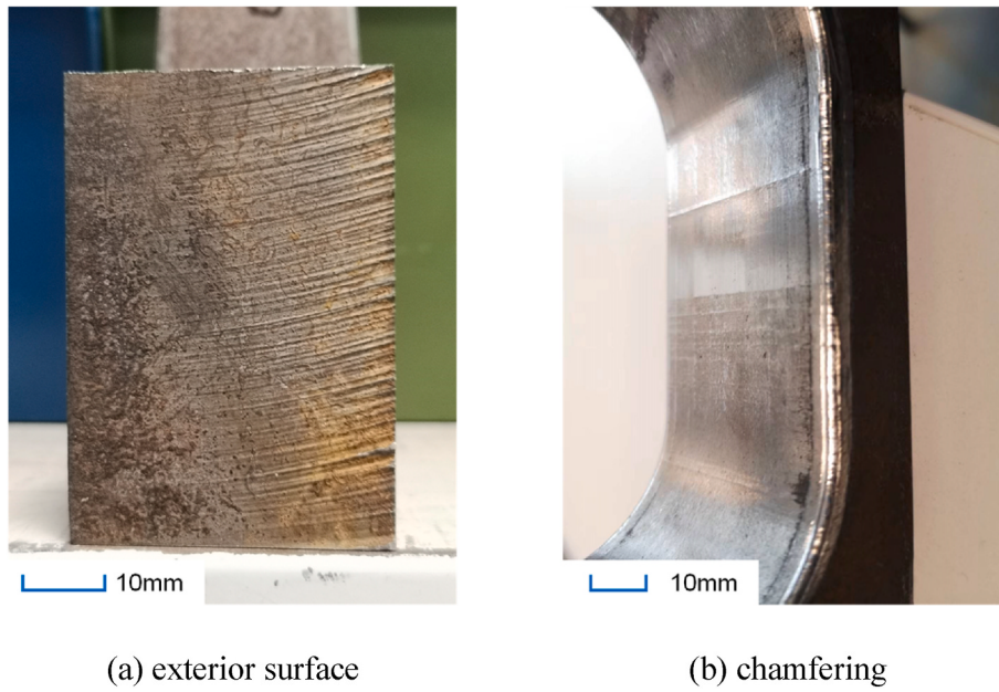
Fig. 13. Manufacturing defects on the as machined holed thick plate.
