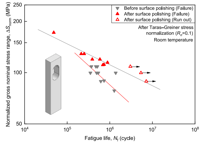
Fig. 10. S-N plots of holed thick plates.
