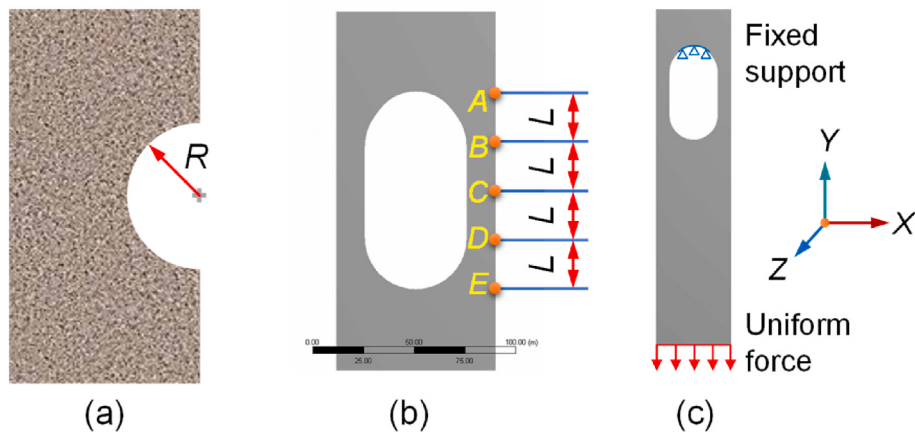
Fig. 15. Details about surface defect (micro notch) simulation.
