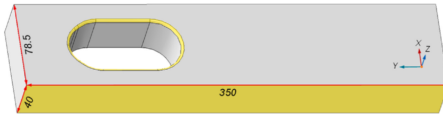
Fig. 3. Three-dimensional view of the central holed thick plate (All dimensions are in mm).
