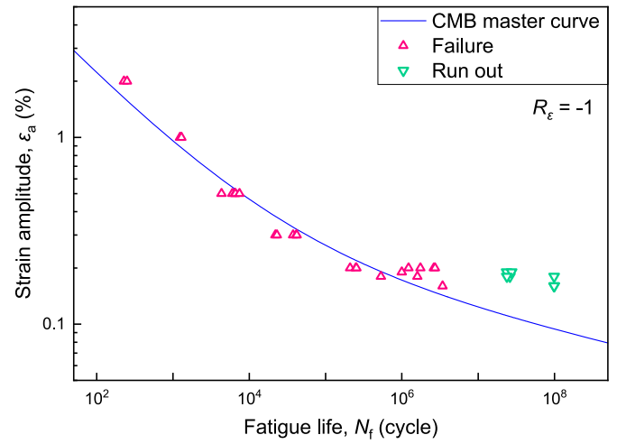
Fig. 7. Fatigue data and CMB master curve.
