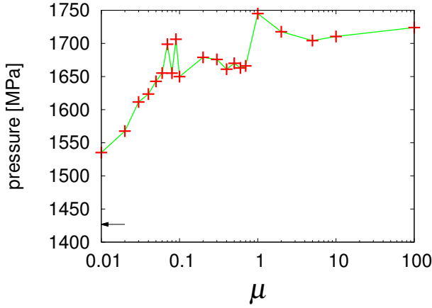
Figure 4.6: Average pressure of the packings ( N = 9261 ) as function of particle coefficient of friction for v_0 = 0.70 and w = 1.5 . The pressure of the frictionless packing is indicated by the arrow. The symbols are data, the lines only a guide to the eye.
