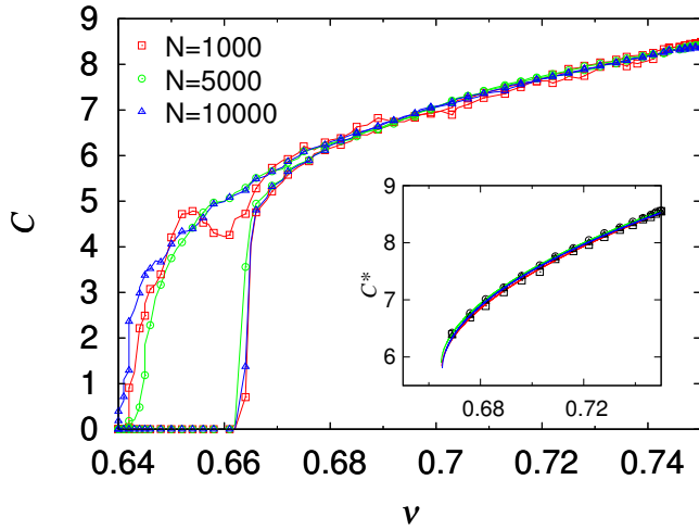
Figure 3.6: Evolution of the coordination number for different system sizes, with w = 3 and D = 0.5 . Inset: Fits of the corrected coordination number C^* according to Eq. (3.4). The red, green and blue lines are the fits for N = 1000 , 5000 and 10000 , respectively.
