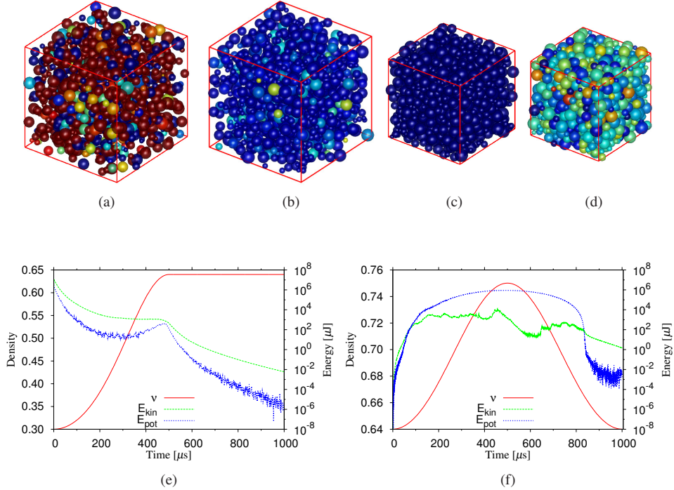
Figure 3.2: Snapshots of the (a) initial (fully) random configuration of the particles ( N = 1000 ) with big (artificial) overlaps and (b) the situation after only 40 \mu seconds compression when all artificial overlaps have disappeared. The color code indicates overlaps of the particles (red: big overlaps, blue: no overlap). (c) Snapshot of the relaxed granular “fluid” with volume fraction v_i = 0.64 . Note that although particles are densely packed they have still practically no overlap, since the volume fraction is below the jamming value v_j . (d) Snapshot of the strongly compressed packing, with v_{\max} = 0.75 using the same color code as in (a), (b) and (c). (e) Evolution of the volume fraction, the potential and the kinetic energy during initial compression and relaxation and (f) the loading-unloading cycle.
