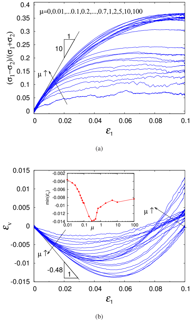
Figure 4.7: Results of DEM triaxial test simulations with different particle coefficients of friction. (a) Deviatoric stress ratio, (b) volumetric strain as a function of axial strain. The inset shows the minimum volumetric strain during axial compression as a function of particle friction.
