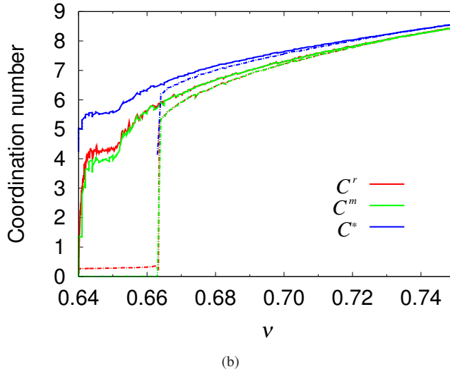
Figure 3.3: (a) Evolution of the fraction of rattlers as function of volume during fraction during unloading for a simulation with N = 10000 , w = 3 , and D = 0.001 . Inset: Fit of Eq. (3.3). (b) Comparison of the coordination numbers computed using the classical C^r , the modified C and the corrected C^* , for the same simulation. The data for loading and unloading are shown by solid and dashed lines, respectively.
