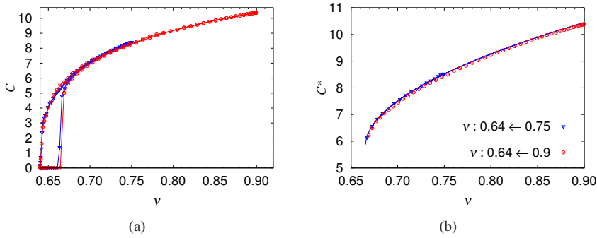
Figure 3.5: (a) Coordination number C as function of volume fraction v for different compression histories. (b) Evolution of C^* during decompression. The solid line is the fit of Eq. (3.4) to the data obtained from the moderately compressed sample ( v : 0.64 \rightleftharpoons 0.75 ).
