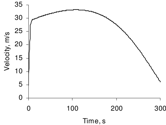
Figure 2b. Second generation Myrabo-like laser propulsion: Velocity
