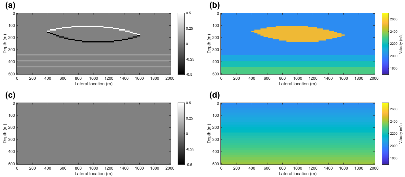
Figure 6 Subsurface model used in this study: (a) true reflectivity model, (b) true velocity model, (c) initial reflectivity model and (d) initial velocity model.
