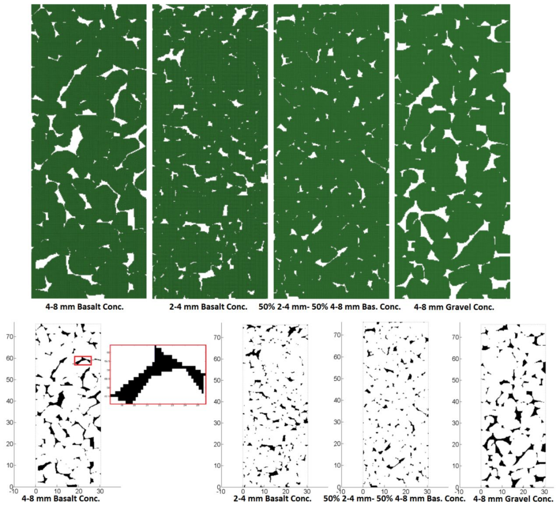
Fig. 13. Determination of pore size distribution
