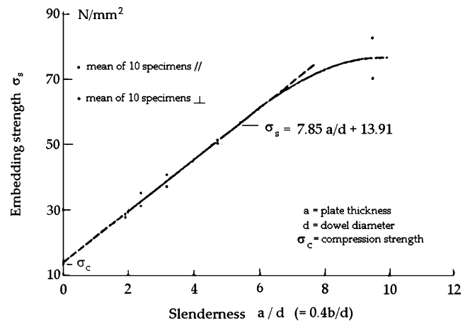
Fig. 4 Embedding strength dependent on a/d ; a = 19 mm
