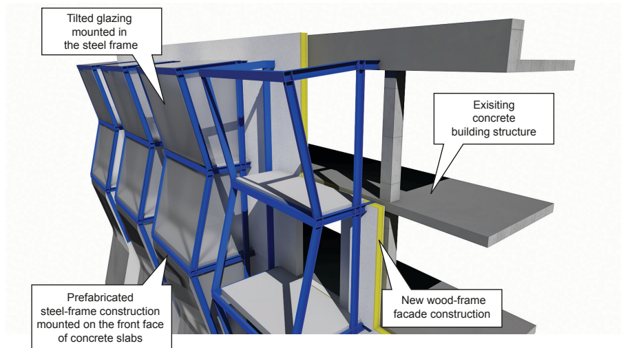
Perspective view of facade concept
