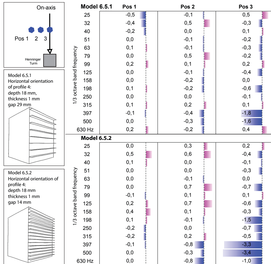
FIGURE 5.25 Frequency distributed level graphs depicting the measured level change for façade models 6.5.1 and 6.5.2 in relation to the planar reference model 1.0.
