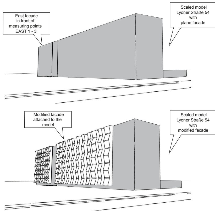
FIGURE 5.31 Measurement variations for the building Lyoner Straße 54.
