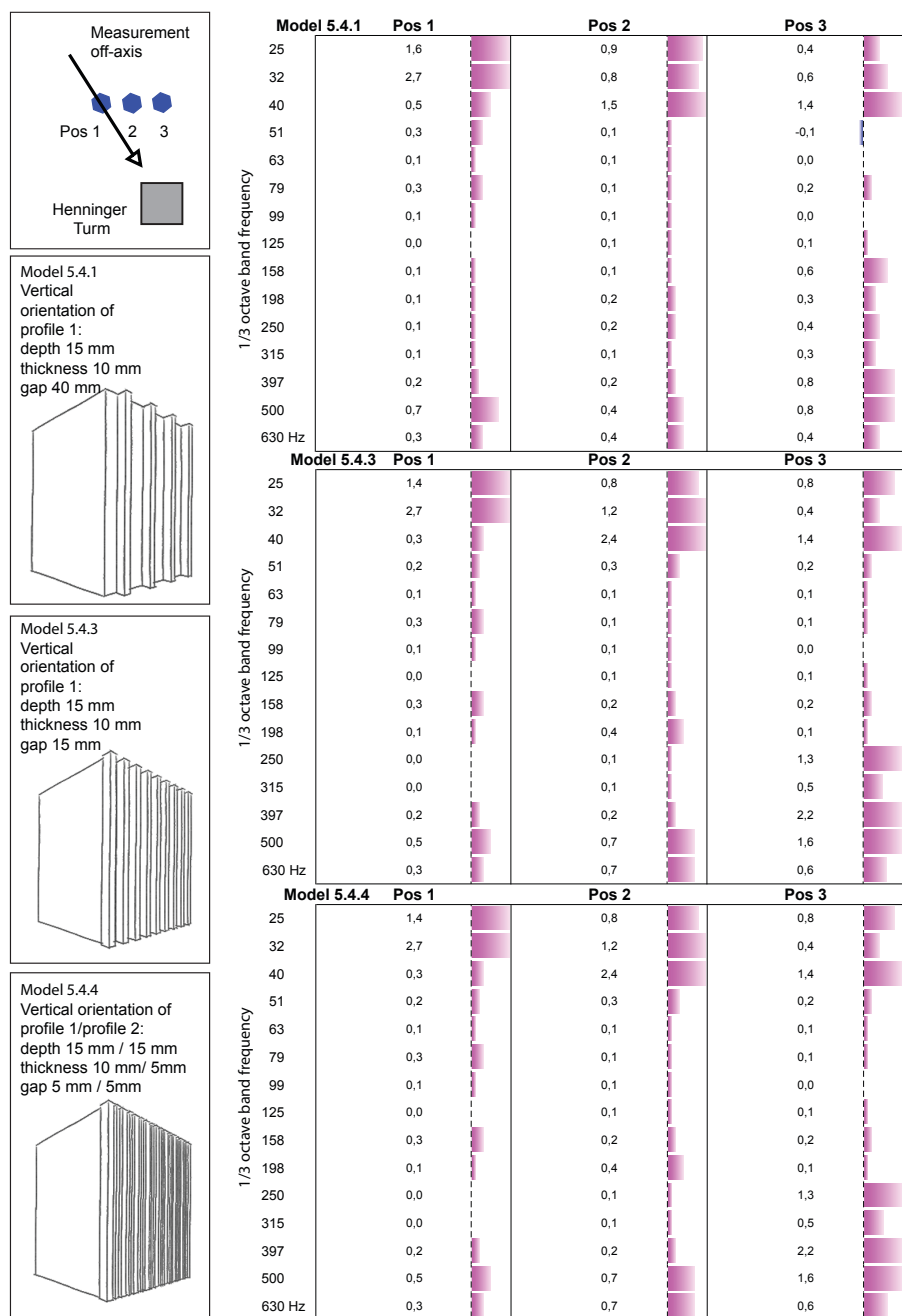
FIGURE 5.28 Measured data off-axis for vertical thick lamellas attached to the model
