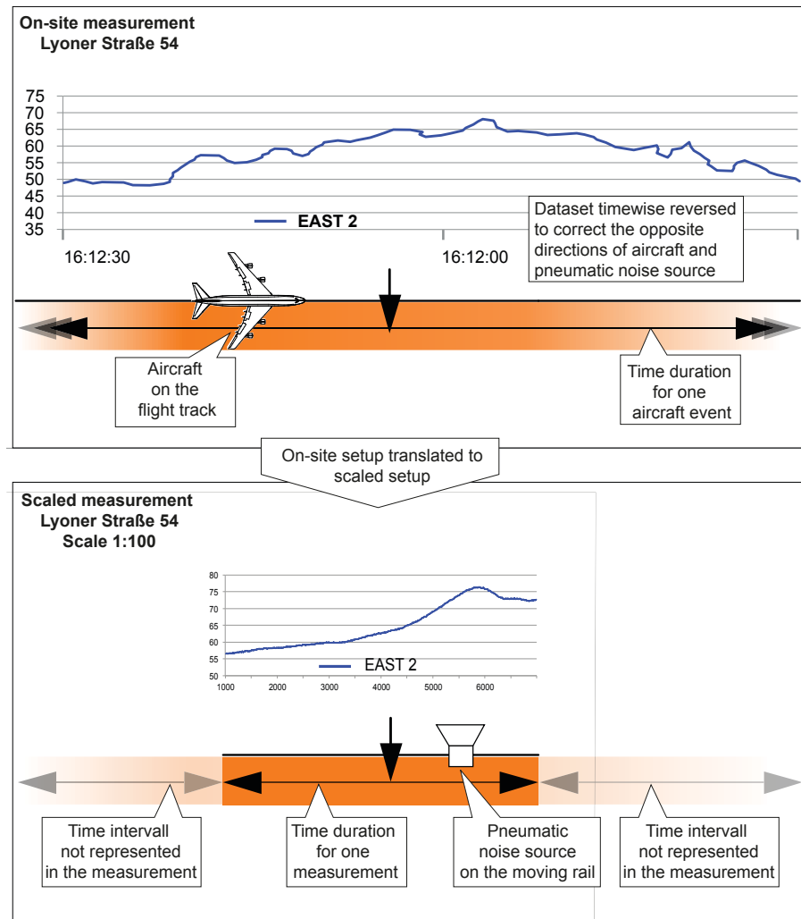
FIGURE 5.41 Level-over-time graph comparison for measuring point EAST 2
