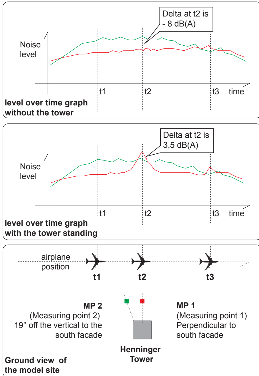
FIGURE 4.15 Correlation graphic of the results from the measurements in relation to the position of the aircraft.
