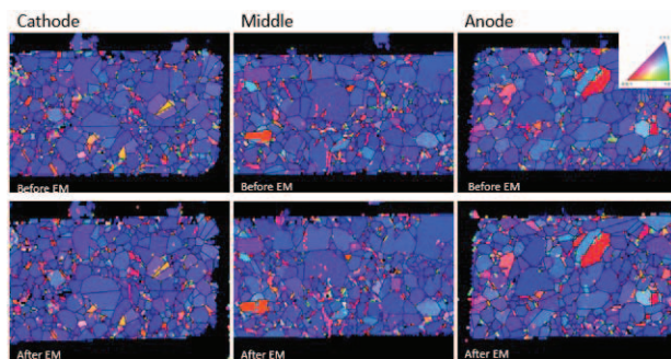
Fig. 5. Crystal orientation maps of 300 °C annealed Cu stripes before and after electromigration.
