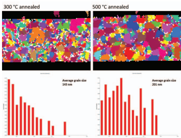
Fig. 4. Grain map and grain size distribution of 300 °C annealed and 500 °C annealed Cu stripes.
