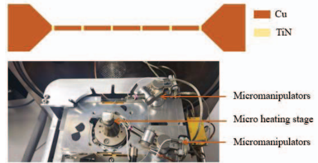
Fig. 1. Schematic diagrams for the test units and in situ setup.
