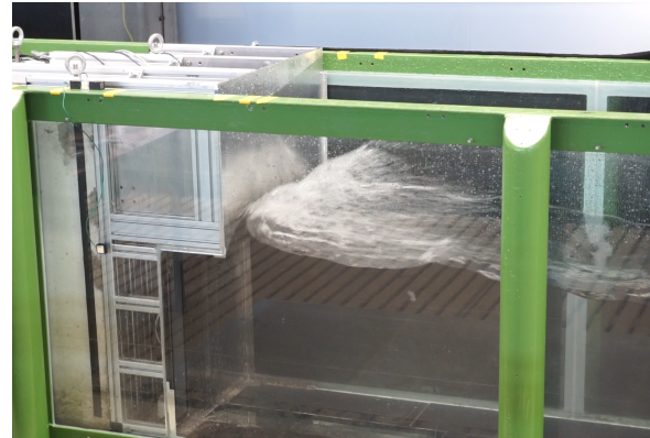
(b) Overhang structure model setup.
