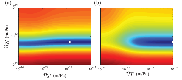
Figure 4: The misfit function in (a) multi-angle P-P AVO inversion and (b) joint P-P + P-S AVO inversion.
